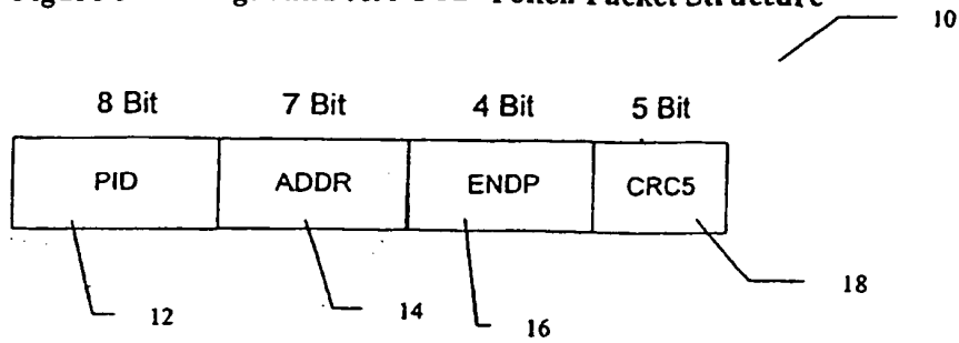
Figure 1 – Background Art USB Token Packet Structure
