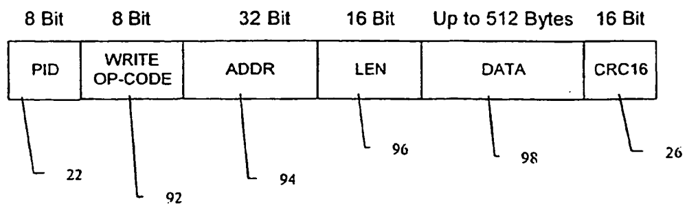
Fig 9 –Write Request Packet
