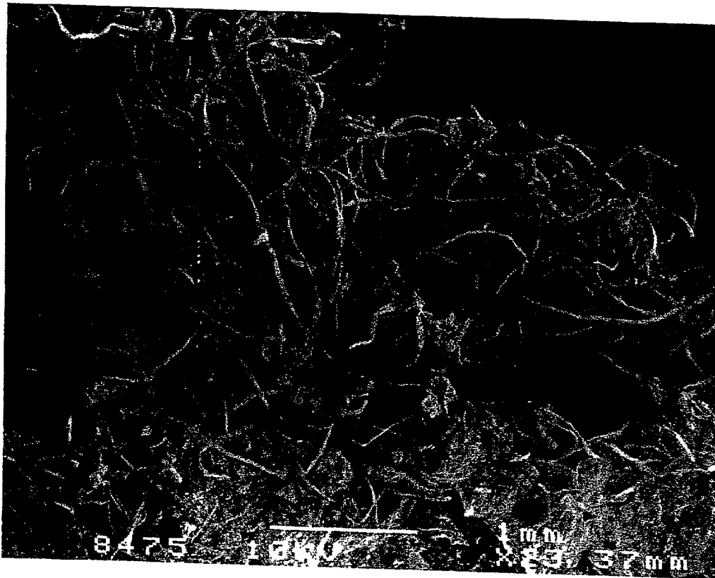
Figure 1 Poor distribution of untreated softwood fibers, added at a volume fraction of 1.7% to a portland cement mortar.
