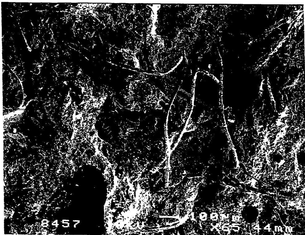
Figure 3 After treatment (beating and adsorption of fly ash), softwood pulp fibers added to mortar at a volume fraction of 1.2% show uniform dispersion. (Compare to untreated fibers in Fig.1)
