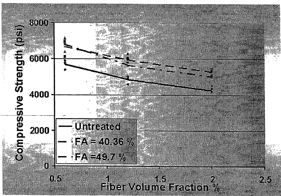
Figure 7 shows a comparative data of the compressive strength of mineral based materials for a period of twenty-eight days. The figure illustrates that treated fibers have an improved compressive strength as compared to the untreated fibers.
