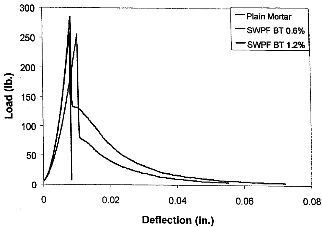
Figure 4 Load vs. deflection curve for unreinforced and treated softwood (SF) fiber reinforced mortars.
