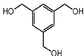
1,3,5-Tri(hydroxymethyl)benzene
