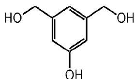
3,5-Di(hydroxymethyl)phenol
