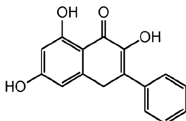
3,5,7-Trihydroxyflavone
