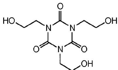
1,3,5-Tris(2-hydroxyethyl)-Cyanuric acid
