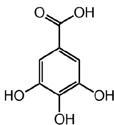
Gallic acid
