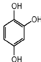
1,2,4-Trihydroxyl-benzene
