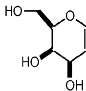
D-Galactal
