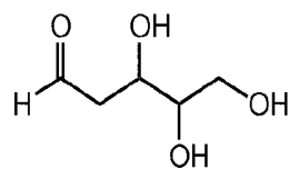
2-Deoxy-D-ribose
