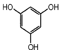
1,3,5-Trihydroxyl-benzene
