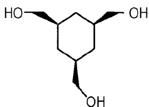
cis-1,3,5-Tri(hydroxymethyl)cyclohexane
