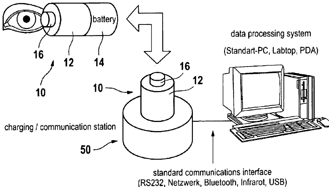
battery-operated hand-held measuring device
