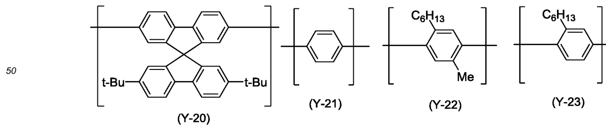
[Chemical Formula 62]
