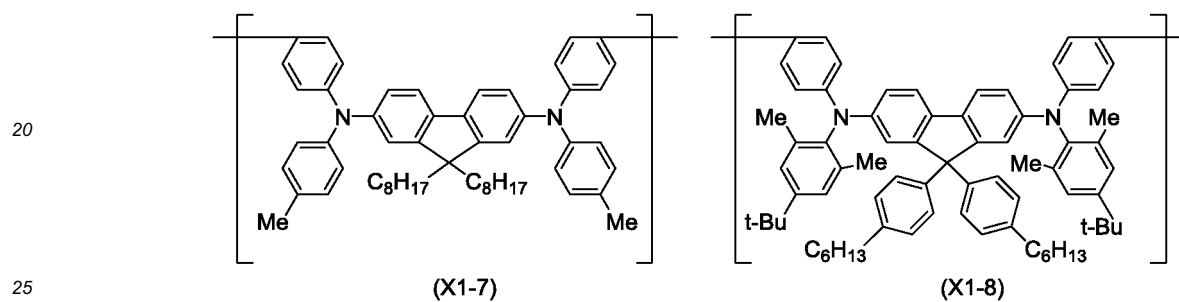
[Chemical Formula 46]
