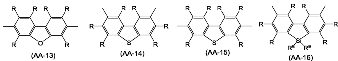
[Chemical Formula 19]
