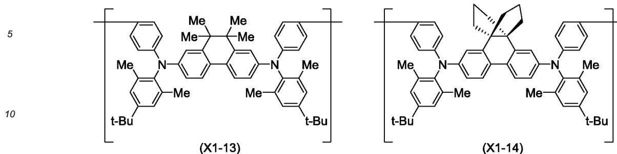
[Chemical Formula 49]
