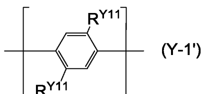
[Chemical Formula 52]
