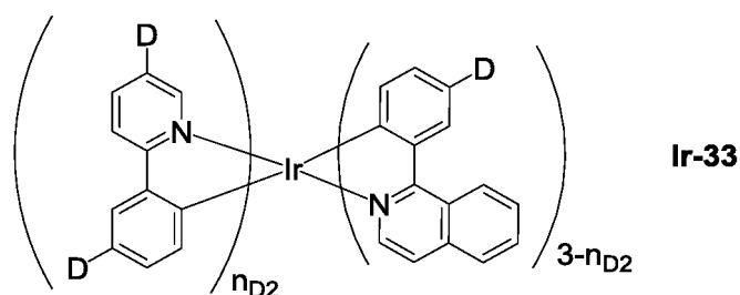
[Chemical Formula 86]
