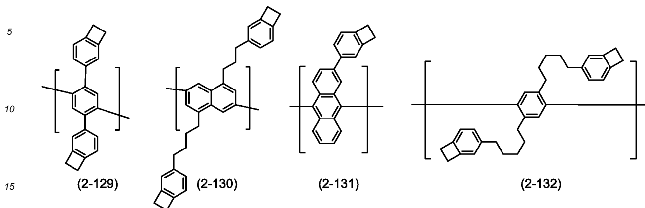
[Chemical Formula 34]
