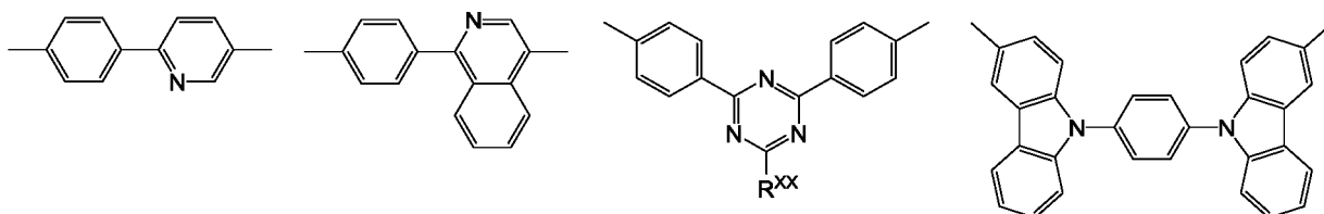
[Chemical Formula 38]
