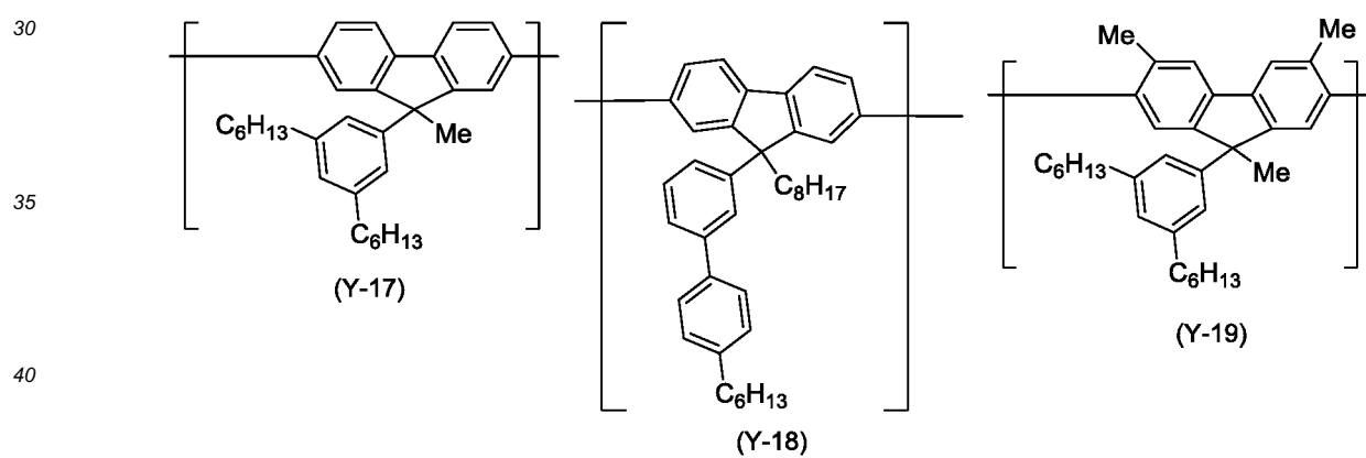
[Chemical Formula 62]
