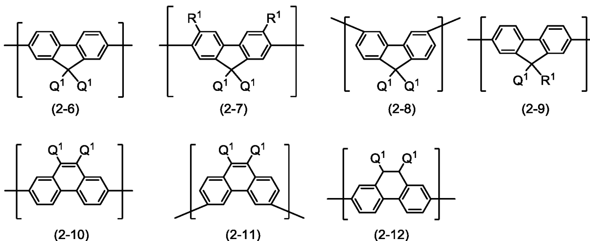
[Chemical Formula 26]
