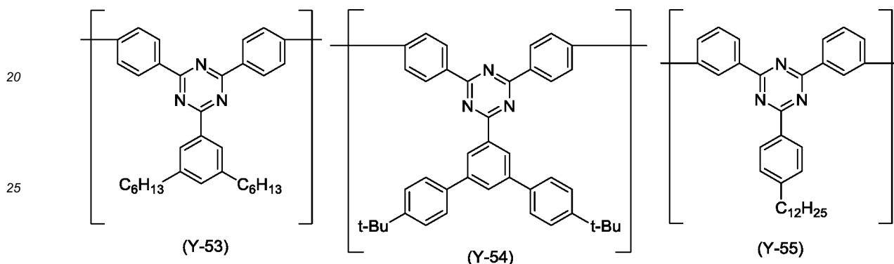
[Chemical Formula 71]
