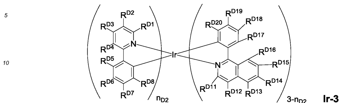
[Chemical Formula 77]
