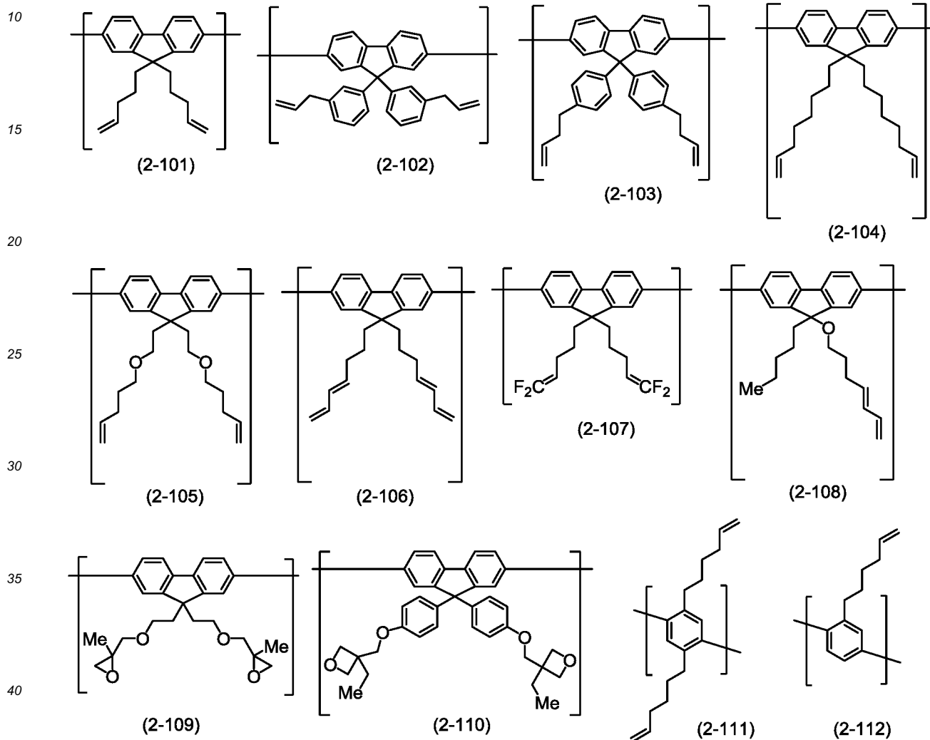
[Chemical Formula 31]
