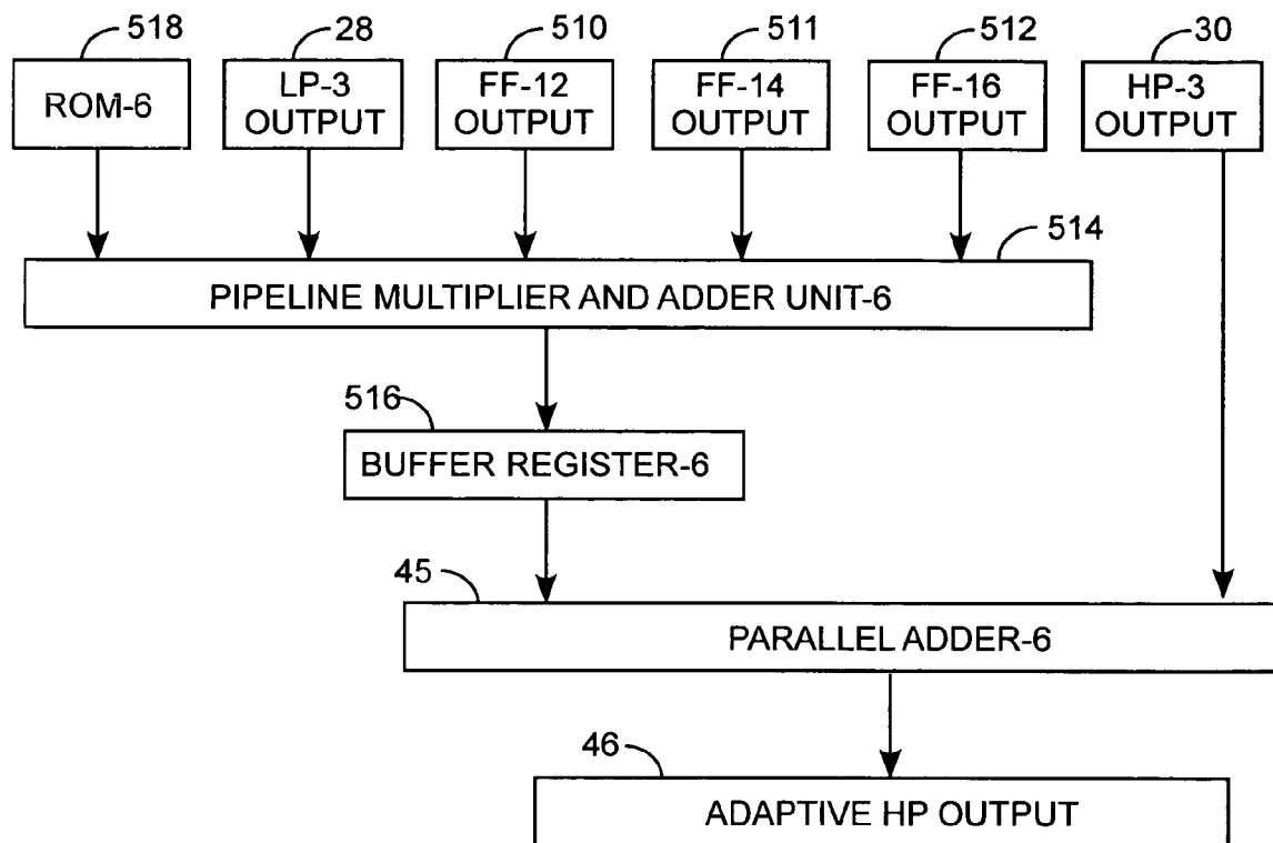
ADAPTIVE LIFTING PIPELINE
