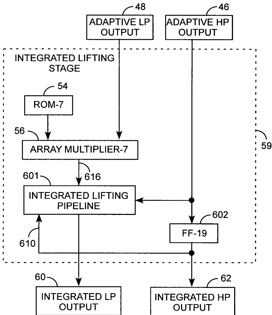
INTEGRATED LIFTING STAGE WAVELET TRANSFORM IMPLEMENTATION
