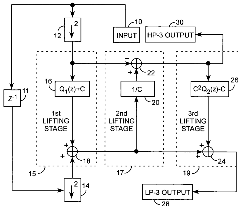
THREE LIFTING STAGE WAVELET TRANSFORM
