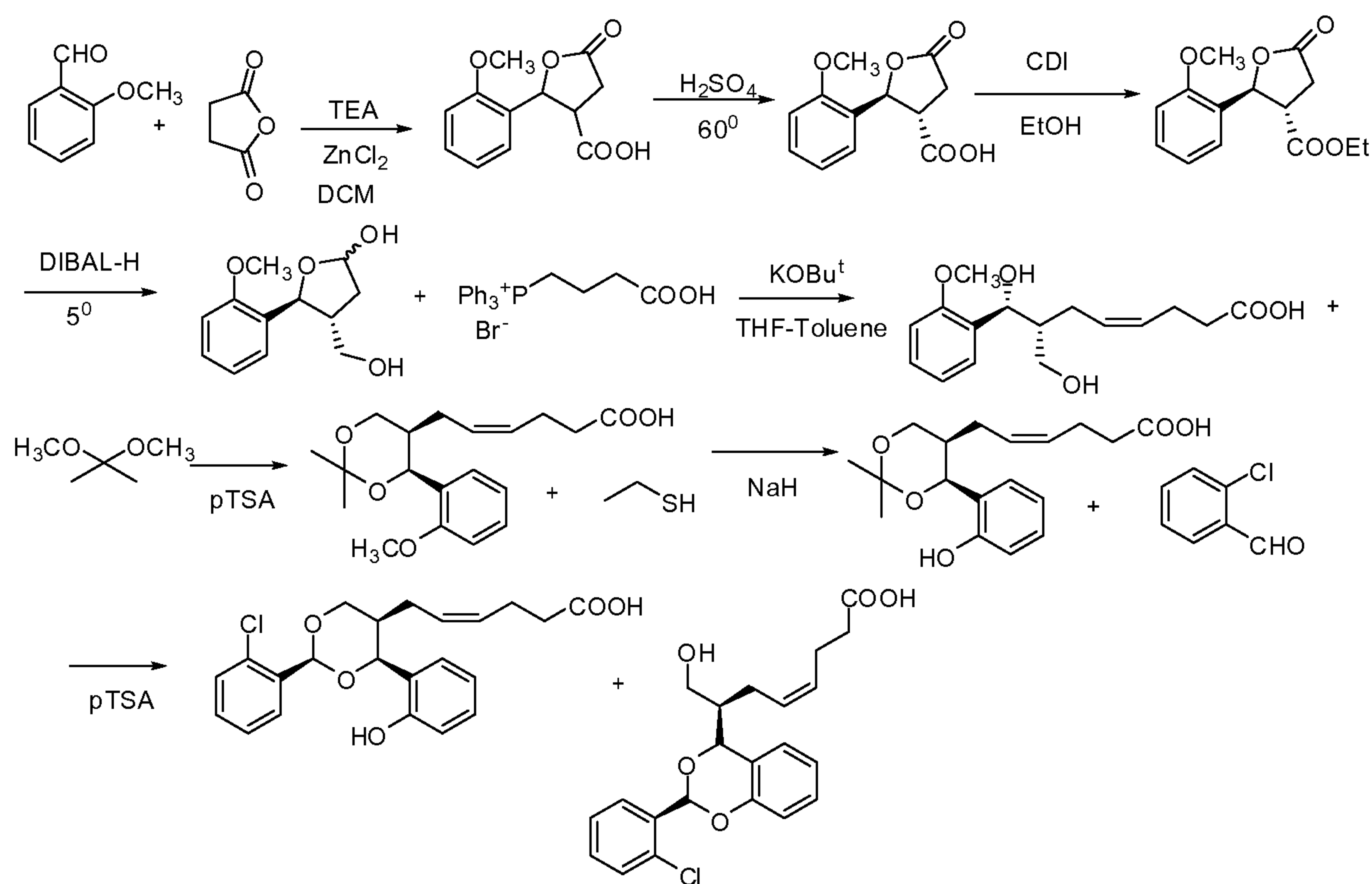
Scheme 2.
