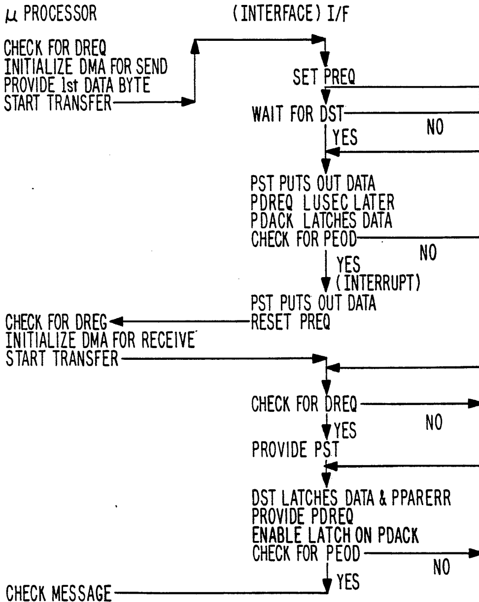
FIG. 5. 6/10 PRINTER INTERFACE STATE MACHINE - FLOW CHART.
