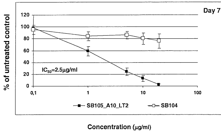
Fig.8. Antiviral activity of SB105_A10 and SB104 on HIV-1 IIIb replication. HIV-1 RNA load analysis
