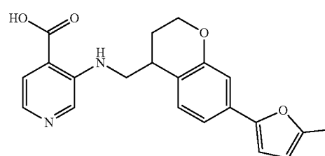
3-([7-(furan-2-yl)-3,4-dihydro-2H-1-benzopyran-4-yl]methyl)amino)pyridine-4-carboxylic acid
