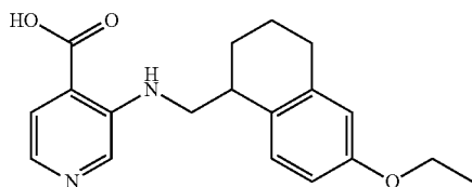
3-({[6-ethoxy-1,2,3,4-tetrahydronaphthalen-1-yl]methyl}amino)pyridine-4-carboxylic acid
