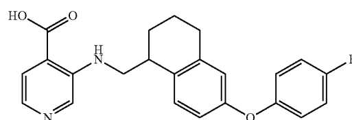
3-([6-(4-fluorophenoxy)-1,2,3,4-tetrahydronaphthalen-1- yl)methyl]amino]pyridine-4-carboxylic acid
