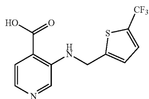
5-[[5-(trifluoromethyl)thiophen-2- yl)methyl]amino]pyridine-4- carboxylic acid
