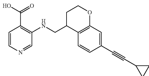
3-([7-(2-cyclopropylethynyl)-3,4-dihydro-2H-1-benzopyran-4-yl]methyl)amino)pyridine-4-carboxylic acid
