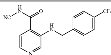
N-cyano-3-(4-(trifluoromethyl)benzylamino)- isonicotinamide
