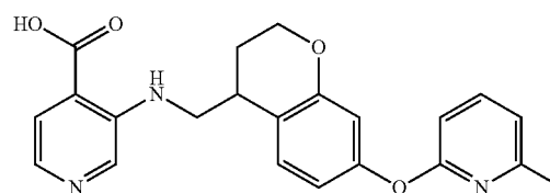
3-([6-[6-methylpyridin-2-yl]oxy]-1,2,3,4-tetrahydronaphthalen-1-yl]methyl)amino)pyridine-4-carboxylic acid
