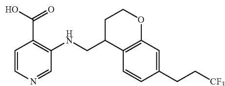
3-([7-(3,3,3-trifluoropropyl)-3,4-dihydro-2H-1-benzopyran-4-yl]methyl)amino)pyridine-4-carboxylic acid
