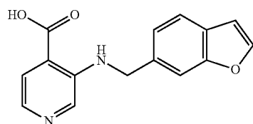
3-[(1-benzofuran-6-ylmethyl)amino]- pyridine-4-carboxylic acid
