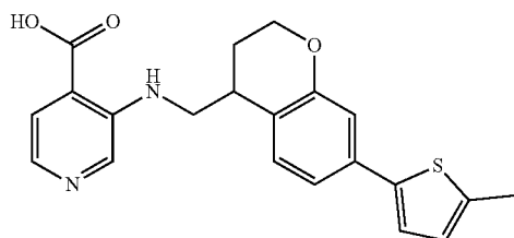
3-([7-(5-methylthiophen-2-yl)-3,4-dihydro-2H-1-benzopyran-4-yl]methyl)amino)pyridine-4-carboxylic acid
