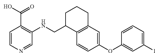
3-([6-(3-fluorophenoxy)-1,2,3,4-tetrahydronaphthalen- 1-yl)methyl]amino]pyridine-4-carboxylic acid
