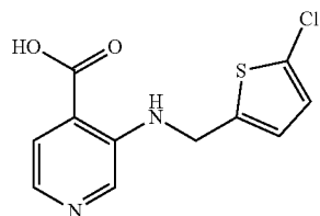
5-[[5-chlorothiophen-2-yl)methyl]- amino]pyridine-4-carboxylic acid
