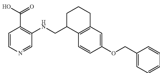
3-({[6-benzyloxy-1,2,3,4-tetrahydronaphthalen-1-yl]methyl}amino)pyridine-4-carboxylic acid
