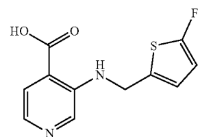
5-[[5-fluorothiophen-2-yl)methyl]- amino]pyridine-4-carboxylic acid
