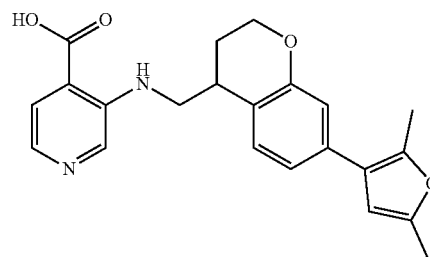
3-([7-(2,5-dimethylfuran-3-yl)-3,4-dihydro-2H-1-benzopyran-4-yl]methyl)amino)pyridine-4-carboxylic acid
