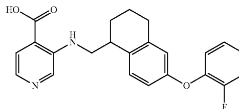
3-([6-(2-fluorophenoxy)-1,2,3,4-tetrahydronaphthalen- 1-yl)methyl]amino]pyridine-4-carboxylic acid
