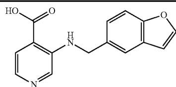
3-[(1-benzofuran-5-ylmethyl)amino]- pyridine-4-carboxylic acid
