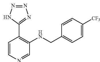
4-(1H-tetrazol-5-yl)-N-(4-(trifluoro- methyl)benzyl)pyridin-3-amine
