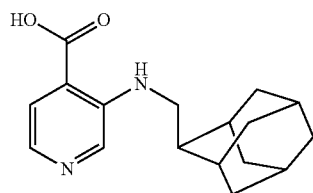
3-[(adamantan-2-ylmethyl)amino]- pyridine-4-carboxylic acid
