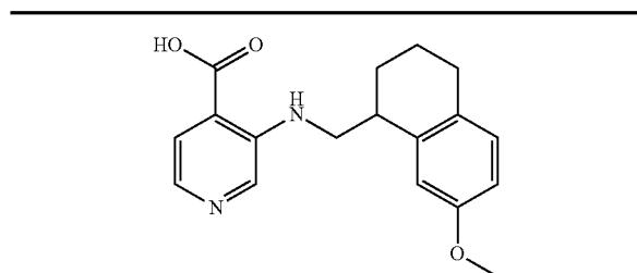
3-({[7-methoxy-1,2,3,4-tetrahydronaphthalen-1-yl]methyl}amino)pyridine-4-carboxylic acid
