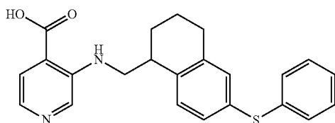
3-({[6-(phenylsulfanyl)-1,2,3,4-tetrahydronaphthalen-1-yl]methyl}amino)pyridine-4-carboxylic acid
