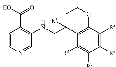
Formula (XIb)
