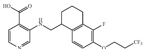
3-([5-fluoro-6-(3,3,3-trifluoropropoxy)-1,2,3,4-tetrahydronaphthalen-1-yl]methyl)amino)pyridine-4-carboxylic acid
