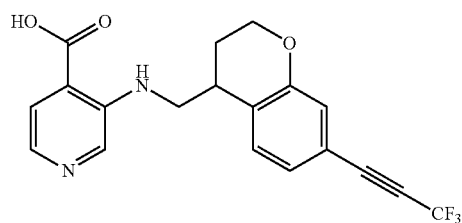
3-([7-(trifluoroprop-1-yn-1-yl)-3,4-dihydro-2H-1-benzopyran-4-yl]methyl)amino)pyridine-4-carboxylic acid
