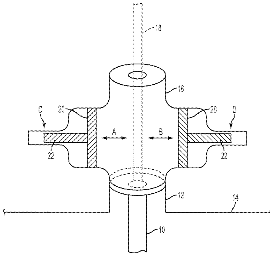
FIG. 1 BACKGROUND ART
