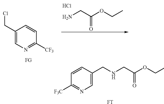
Scheme 103: Prepared Via Method XLXVI:
