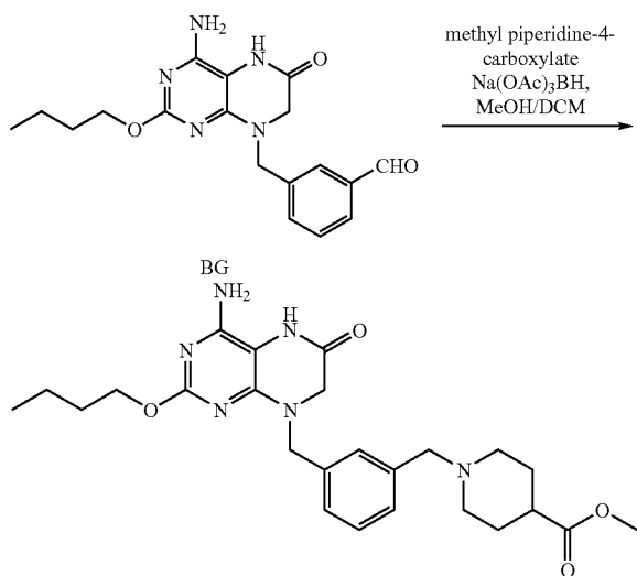
Example 54
