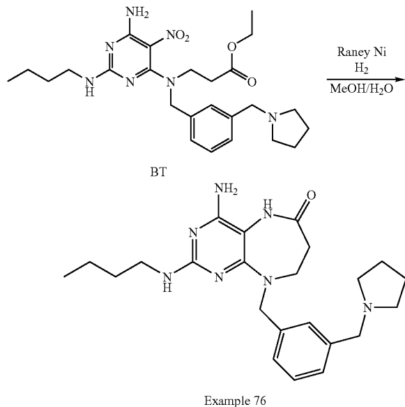
Scheme 67: Example 76, Prepared using Method XIV:
