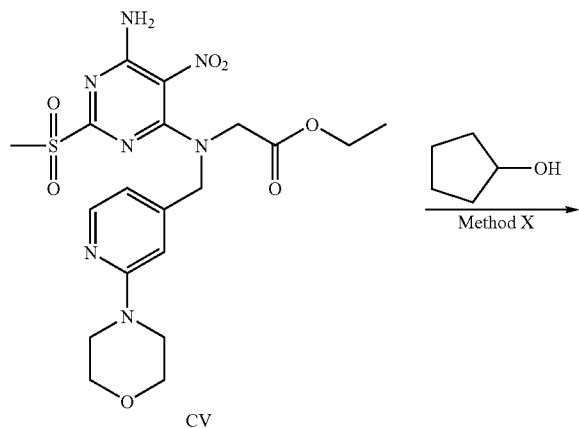
Scheme 58: Example 69, Method X followed by Method XII
