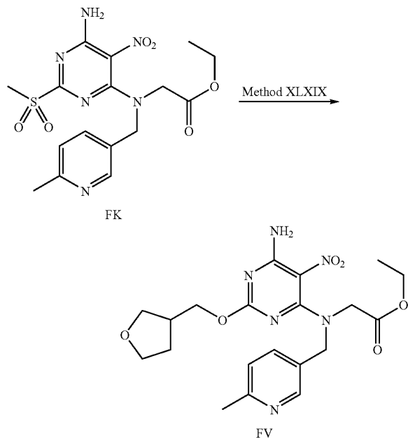
Scheme 114: Prepared Via Method XLXIX
