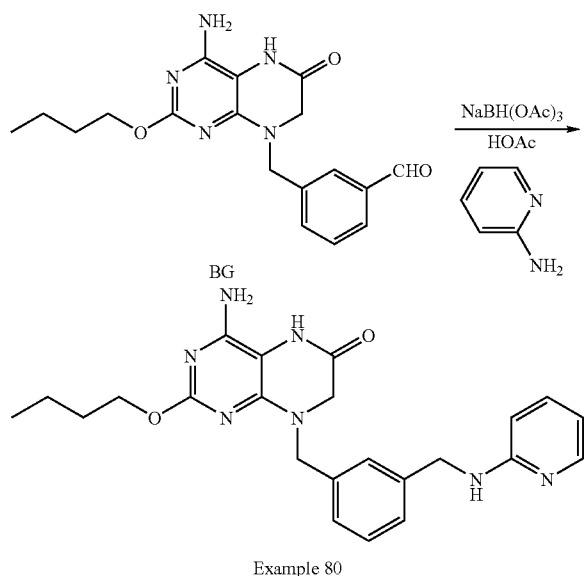
Scheme 73: Example 80, Made Using XXI:
