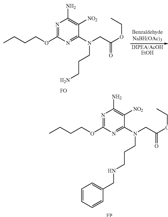
Scheme 106:
