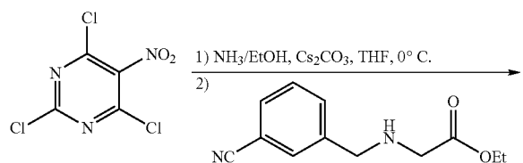
Scheme 49
