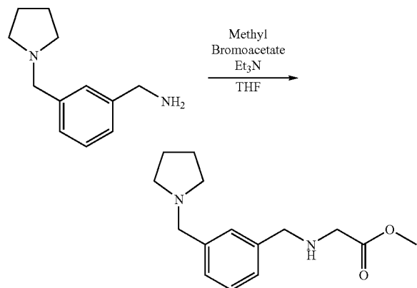
Scheme 20
