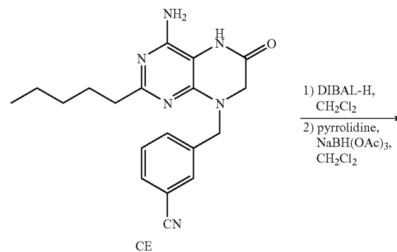
Scheme 53: Example 53
