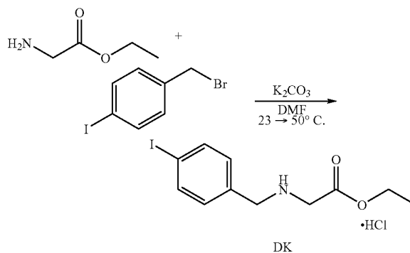
Scheme 77
