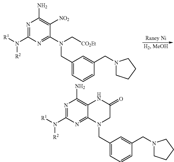
Scheme 17
