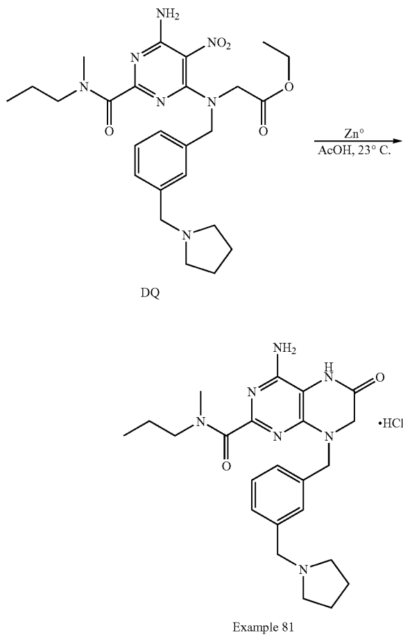
Scheme 84: Example 81
