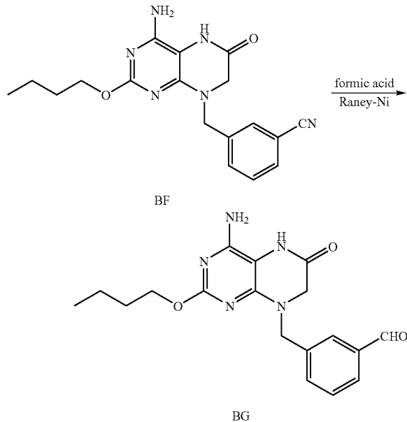
Scheme 24
