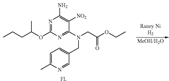
Scheme 101:
