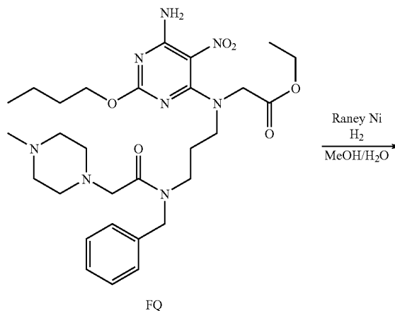
Scheme 108: Example 110: Method XLXX:
