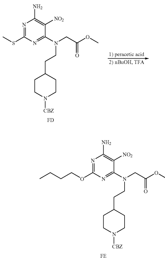
Scheme 93
