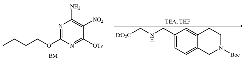
Scheme 89:
