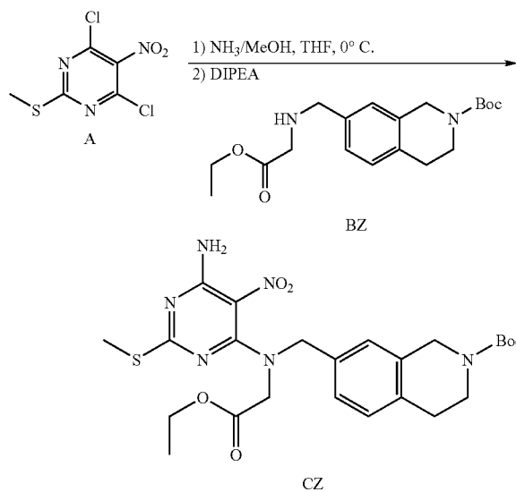
Scheme 59: Prepared Via Method XVII:
