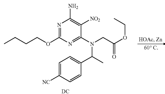
Scheme 64: Compound DD Prepared Via Method XXXIII:
