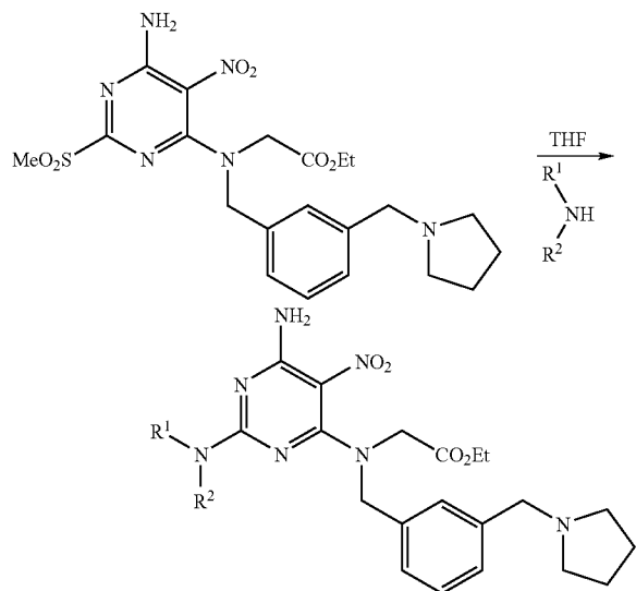
Scheme 16
