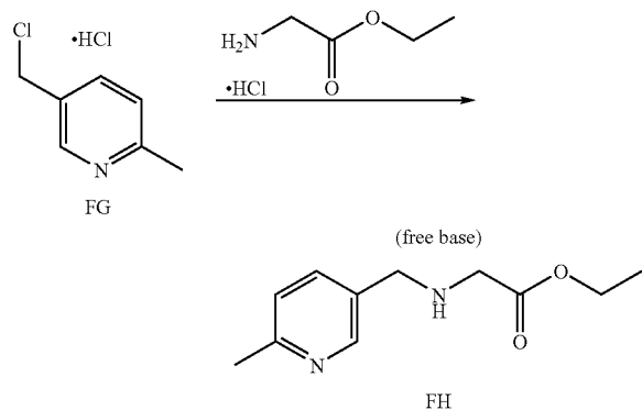
Scheme 97
