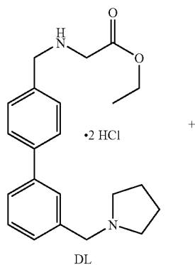
Scheme 86
