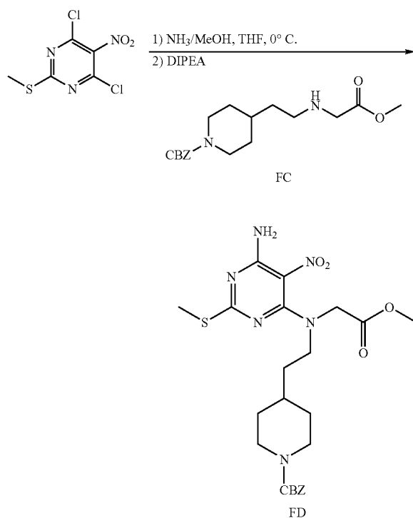
Scheme 92
