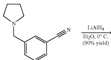
Scheme 5
