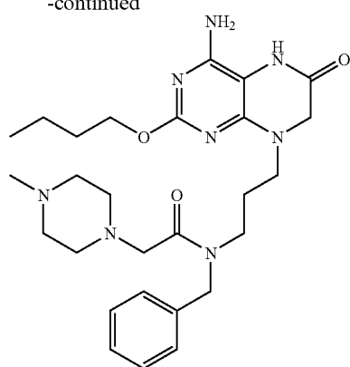
Example 110
