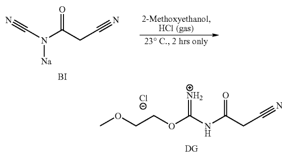
Scheme 74
