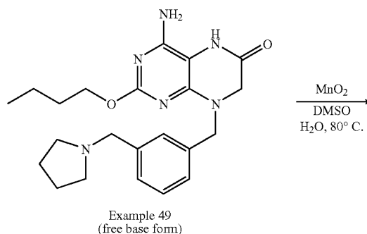
Scheme 87
