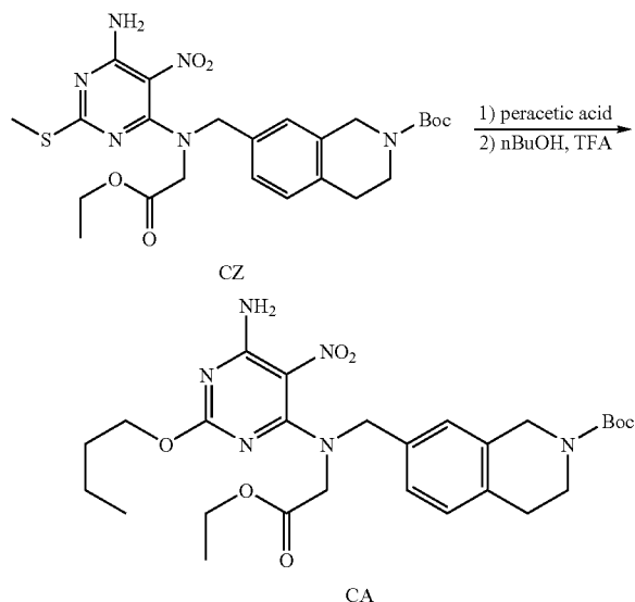
Scheme 60: Compound CA Prepared Via Method XVIII:
