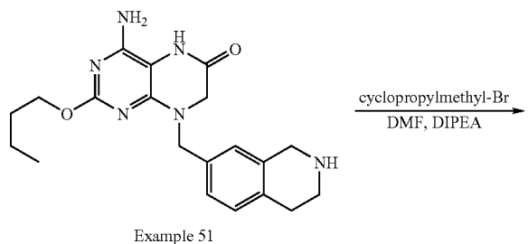
Scheme 61: Example 70, Method XLVIII
