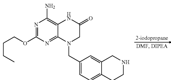
Example 51
