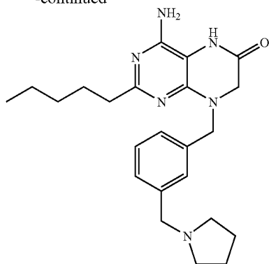
Example 53
