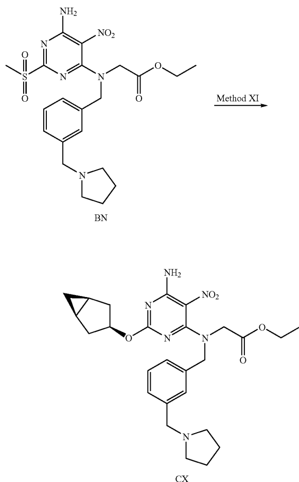
Scheme 56: Prepared Via Method XI
