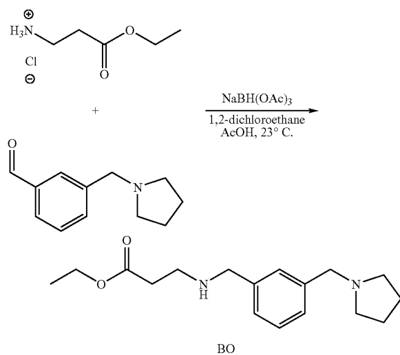
Scheme 33
