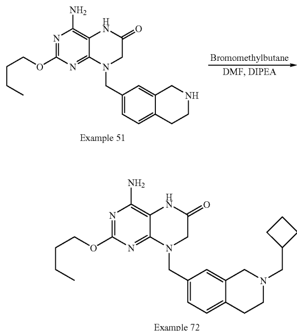
Scheme 63: Example 72, Method XLVIII:
