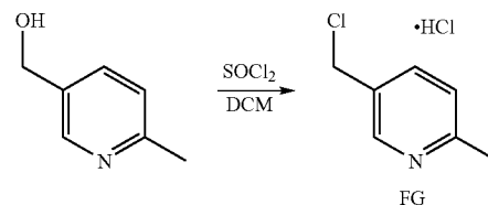
Scheme 96:
