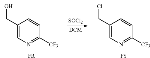
Scheme 102: Prepared Via Method XLXV:
