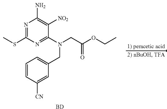
Scheme 22
