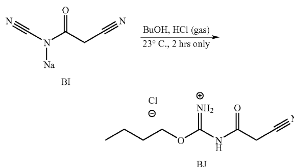
Scheme 28
