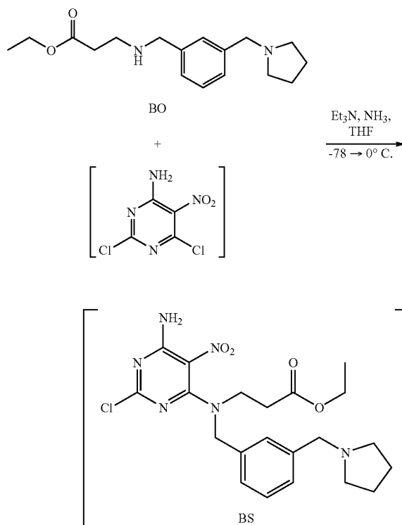
Scheme 40
