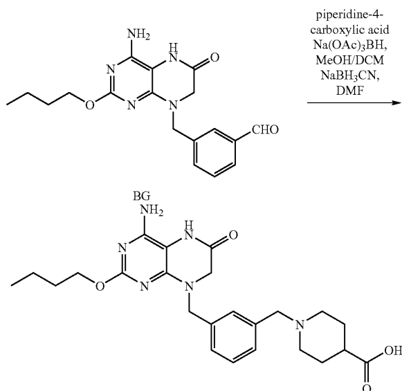
Example 75
