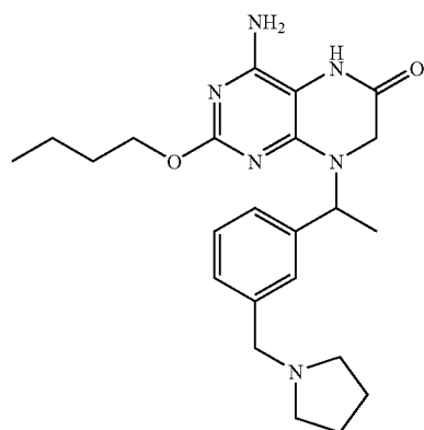
Example 73
