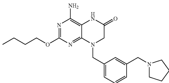
Scheme 28
