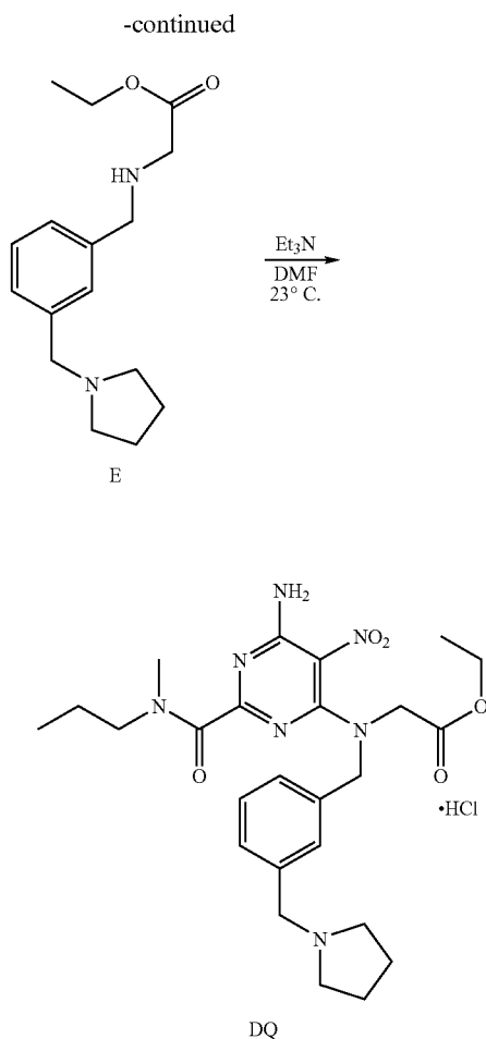
Scheme 84: Example 81
