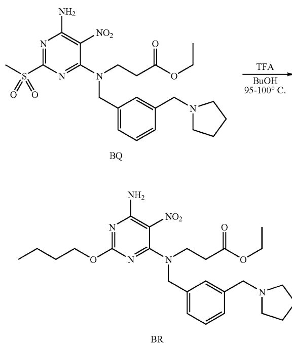
Scheme 37
