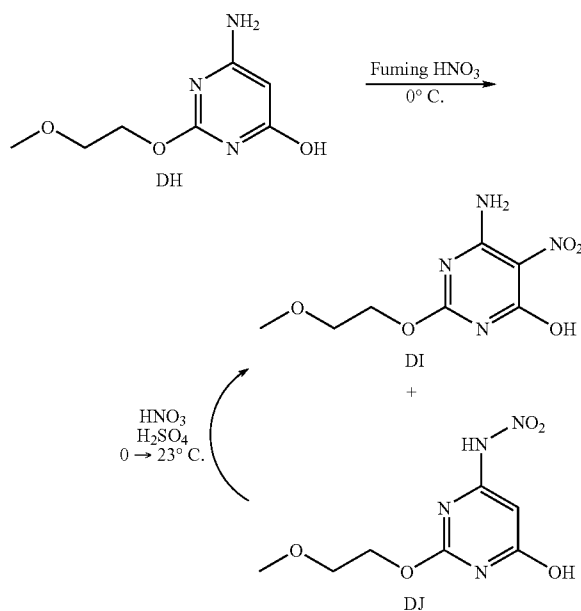
Scheme 76
