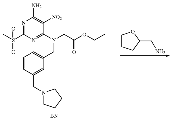
Scheme 68: Compound DE Prepared Via Method XIII
