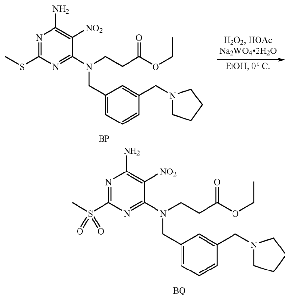
Scheme 36
