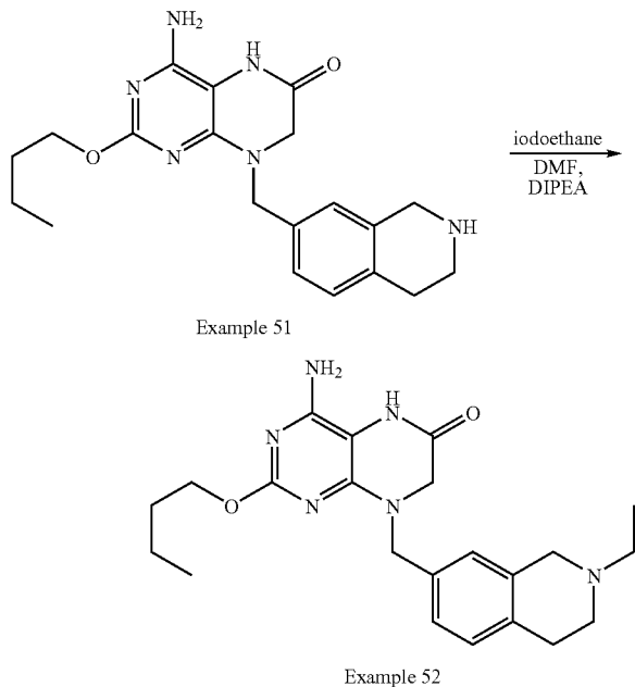
Scheme 48: Example 52
