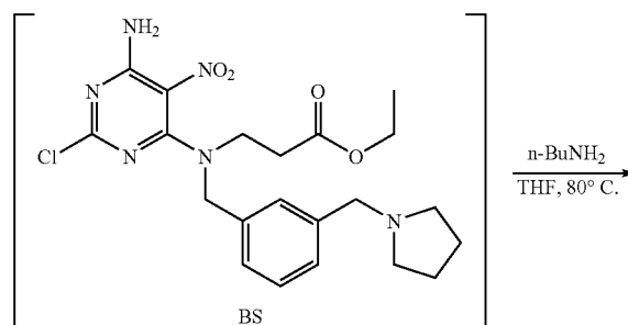
Scheme 41
