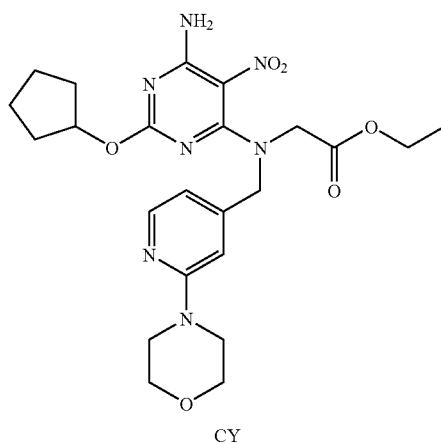
Scheme 59: Prepared Via Method XVII:
