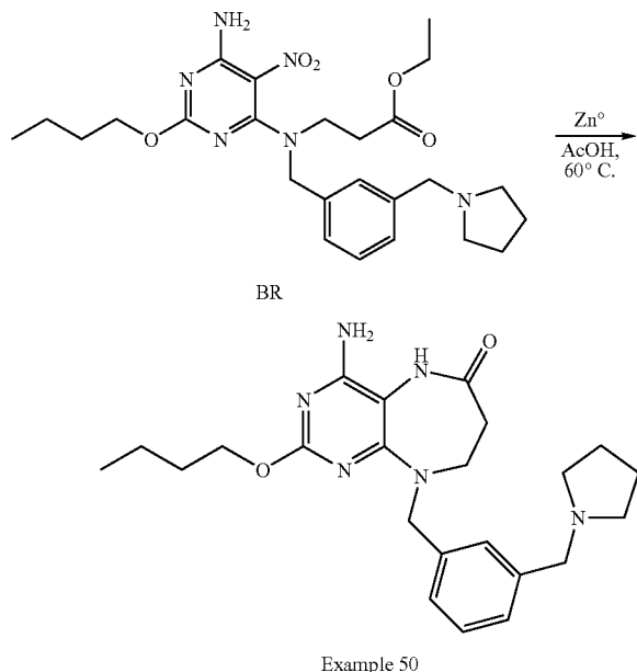
Scheme 38: Example 50
