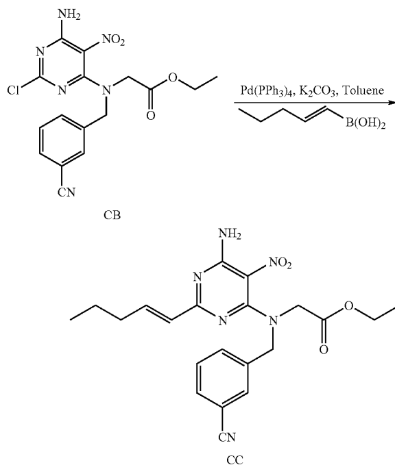
Scheme 50
