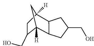
octahydro-4,7-methano-1H-indenedimethanol (TCD alcohol DM)
