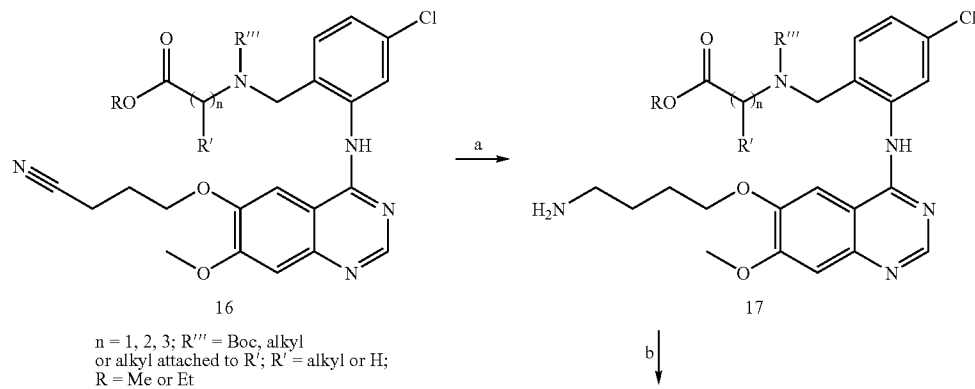
Scheme 10b.
