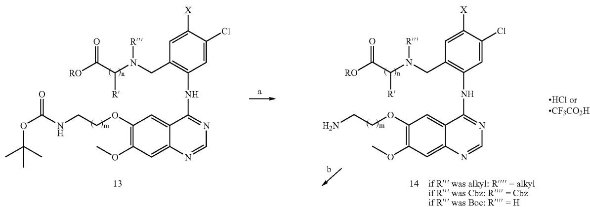
Scheme 9b.
