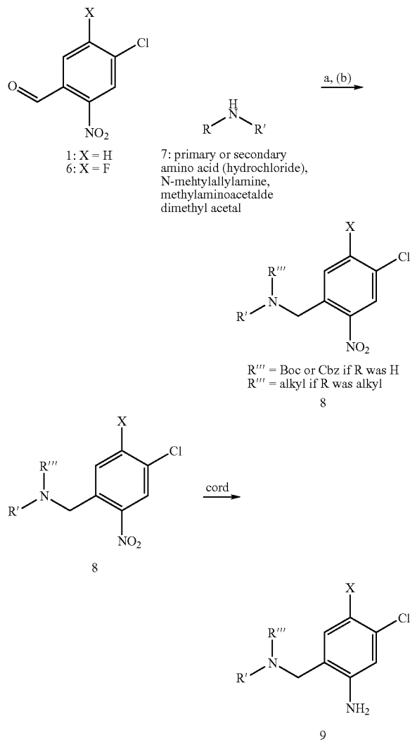
Scheme 5b.
