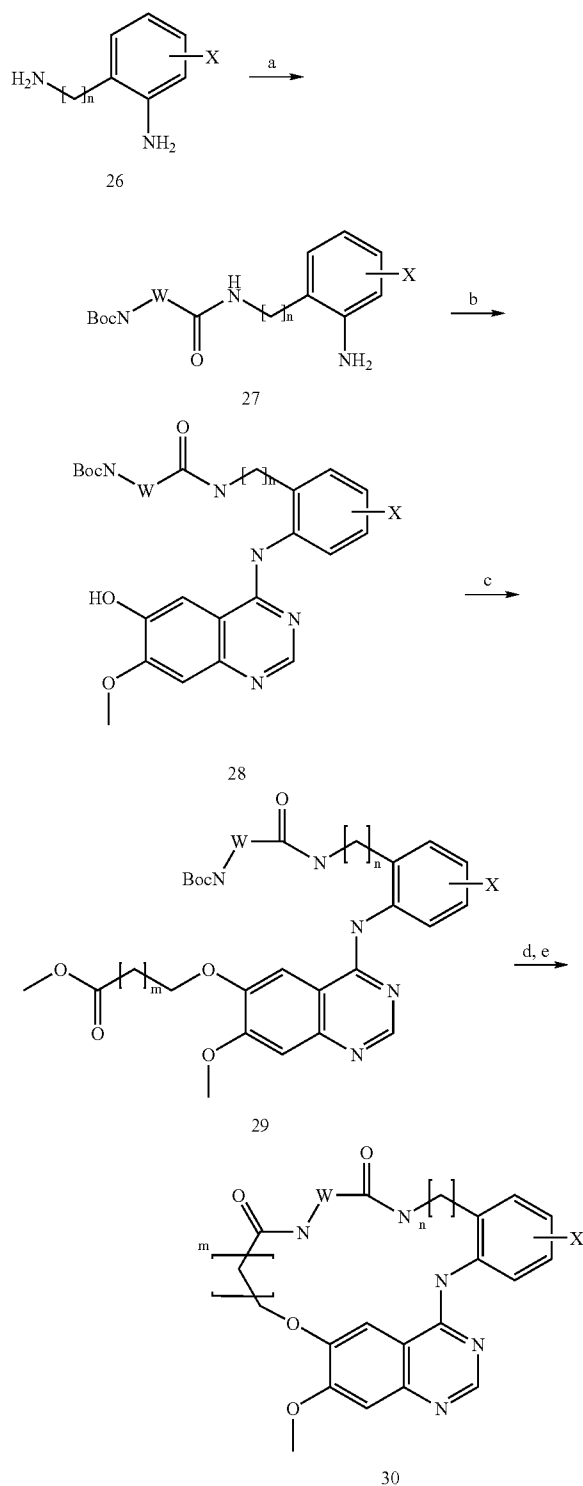
Scheme 12
