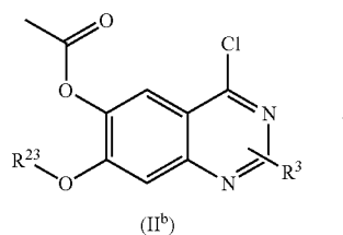
Scheme 13
