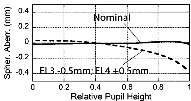
Variable Soft Focus Type 3: Move Elements 3 and 4
