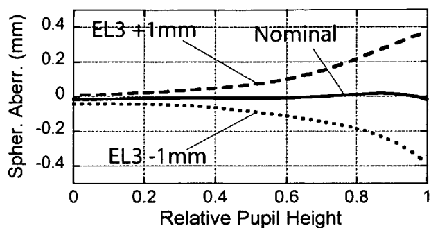
Variable Soft Focus Type 1: Move Element 3
