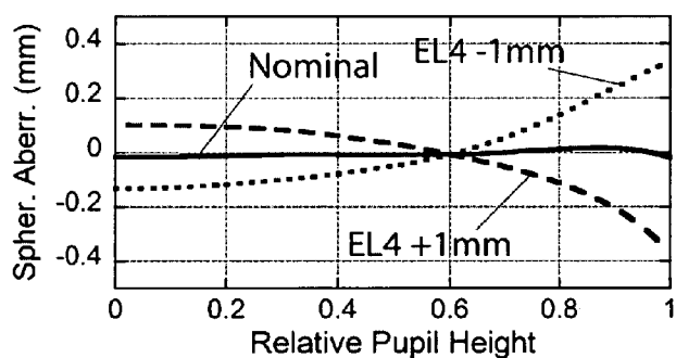
Variable Soft Focus Type 2: Move Element 4
