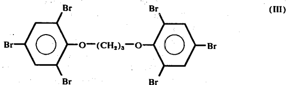
1,3-bis(2,4,6-tribromophenoxy) propane
