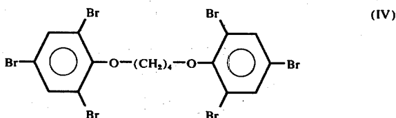
1,4-bis(2,4,6-tribromophenoxy) butane
