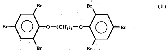
1,2-bis(2,4,6-tribromophenoxy) ethane
