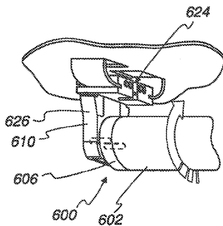
Fig. 60 Prior Art
