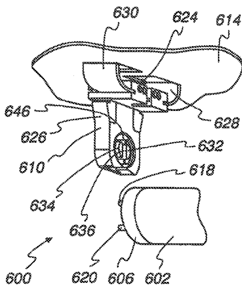
Fig. 56 Prior Art
