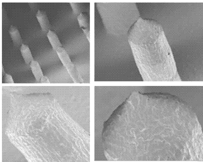
FIG. 21B SEM images of the individual needles
