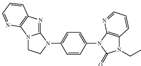
134a) ethyl N-(3-nitropyridin-2-yl)glycinate
