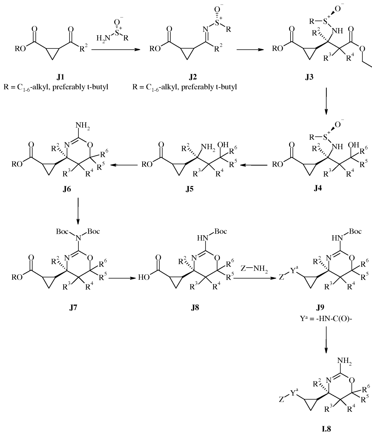
Scheme J: Synthesis of compounds of formula I.8 .
