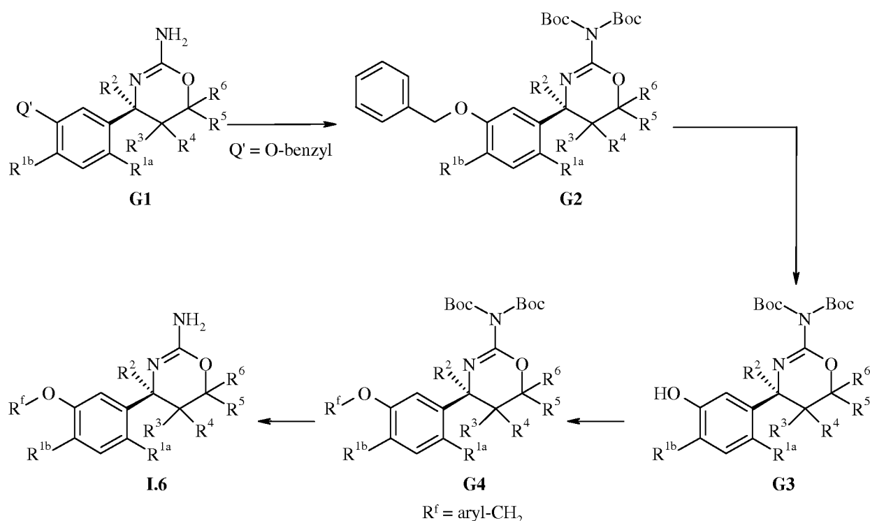
Scheme G: Synthesis of compounds of formula I.6 .
