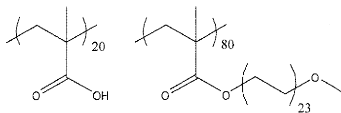
Polymer (1)
