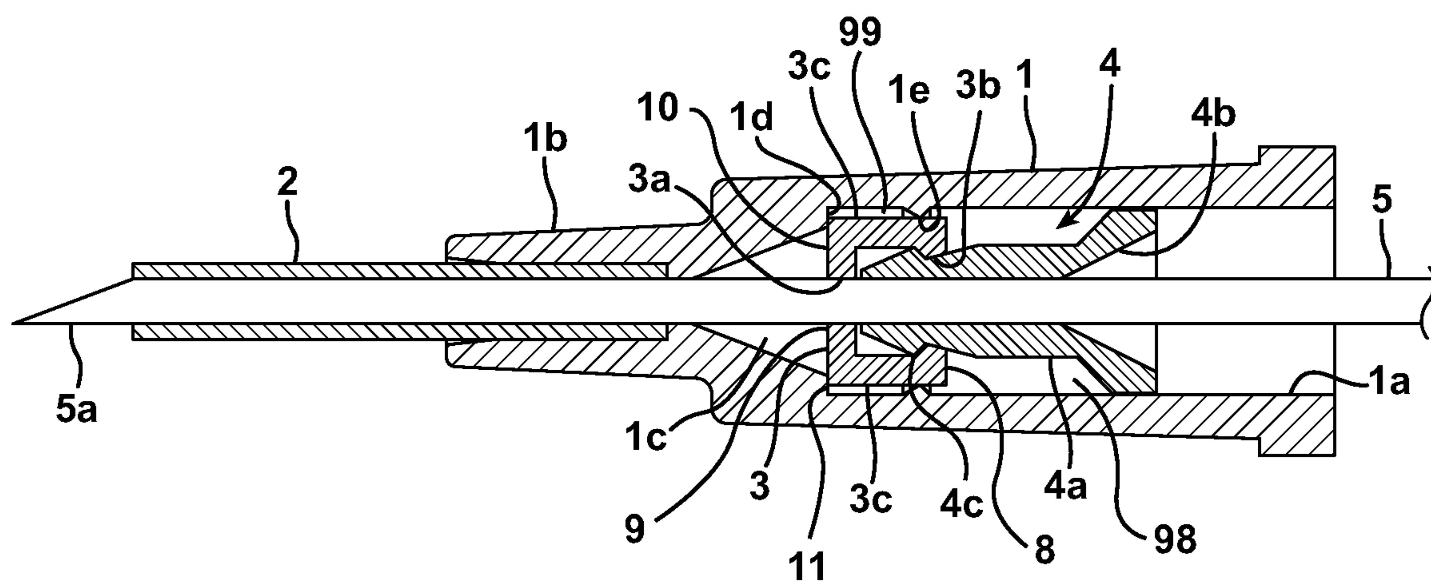
FIG. 1 Prior Art
