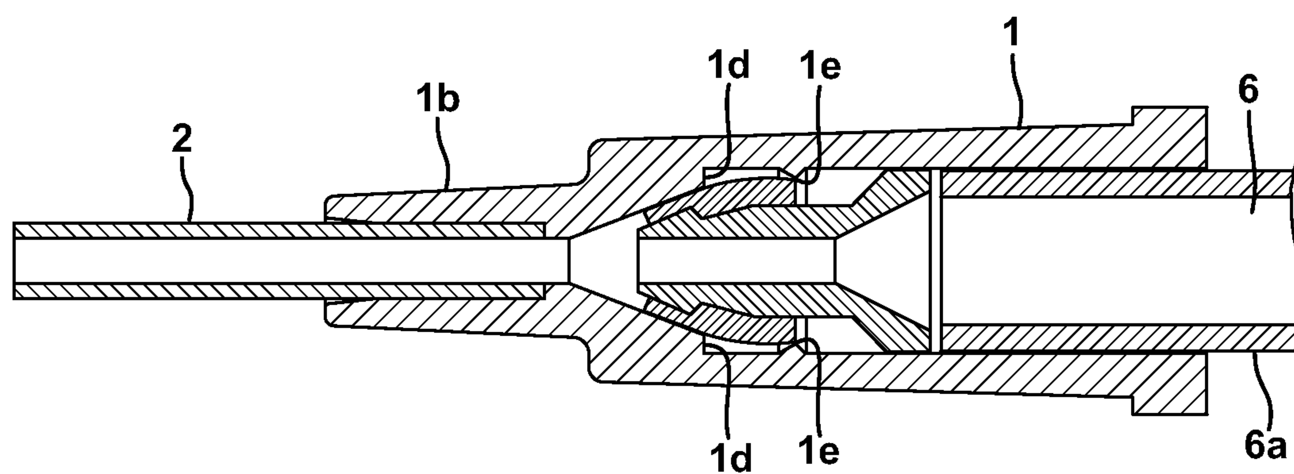
FIG. 3 Prior Art
