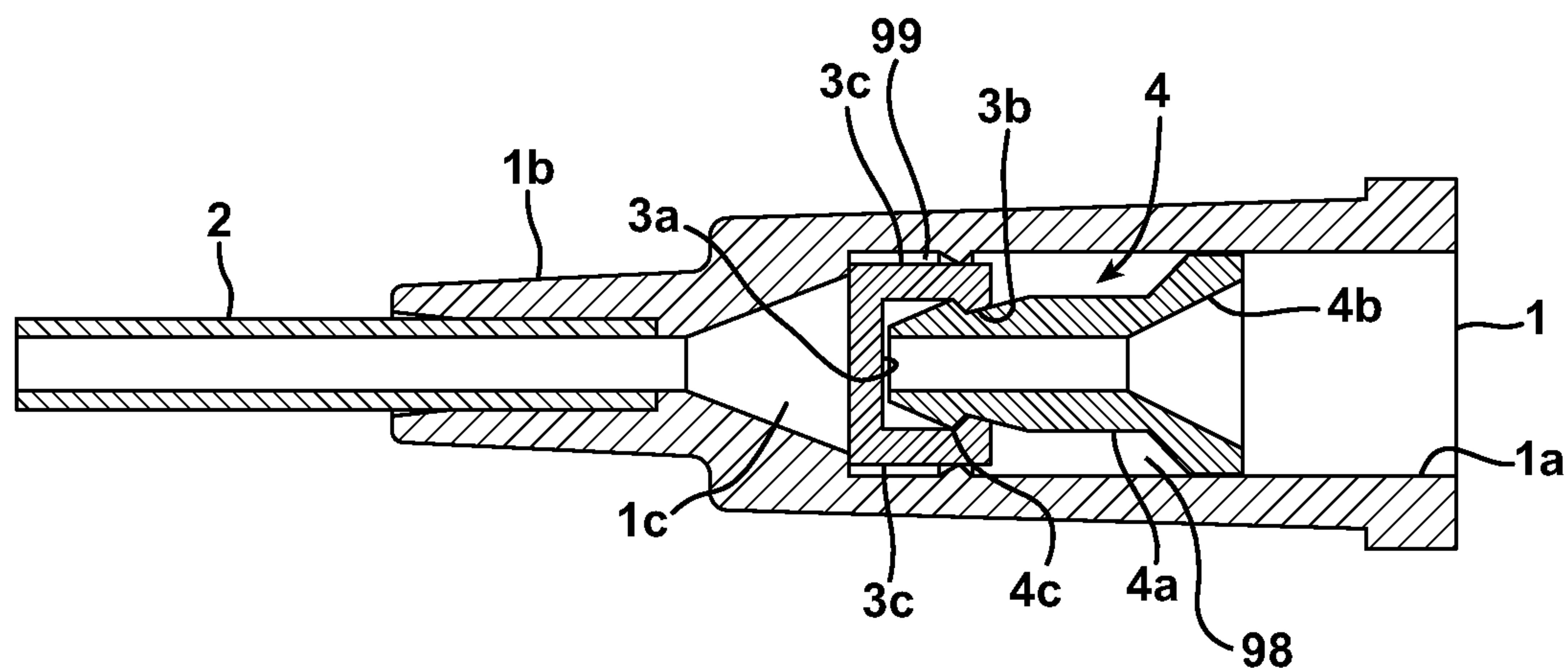
FIG. 2 Prior Art
