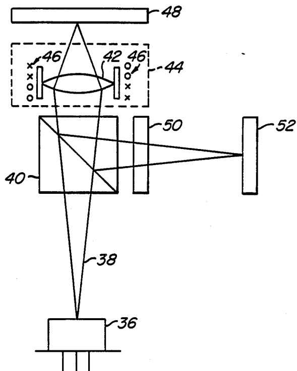
(PRIOR ART) FIG. 2.
