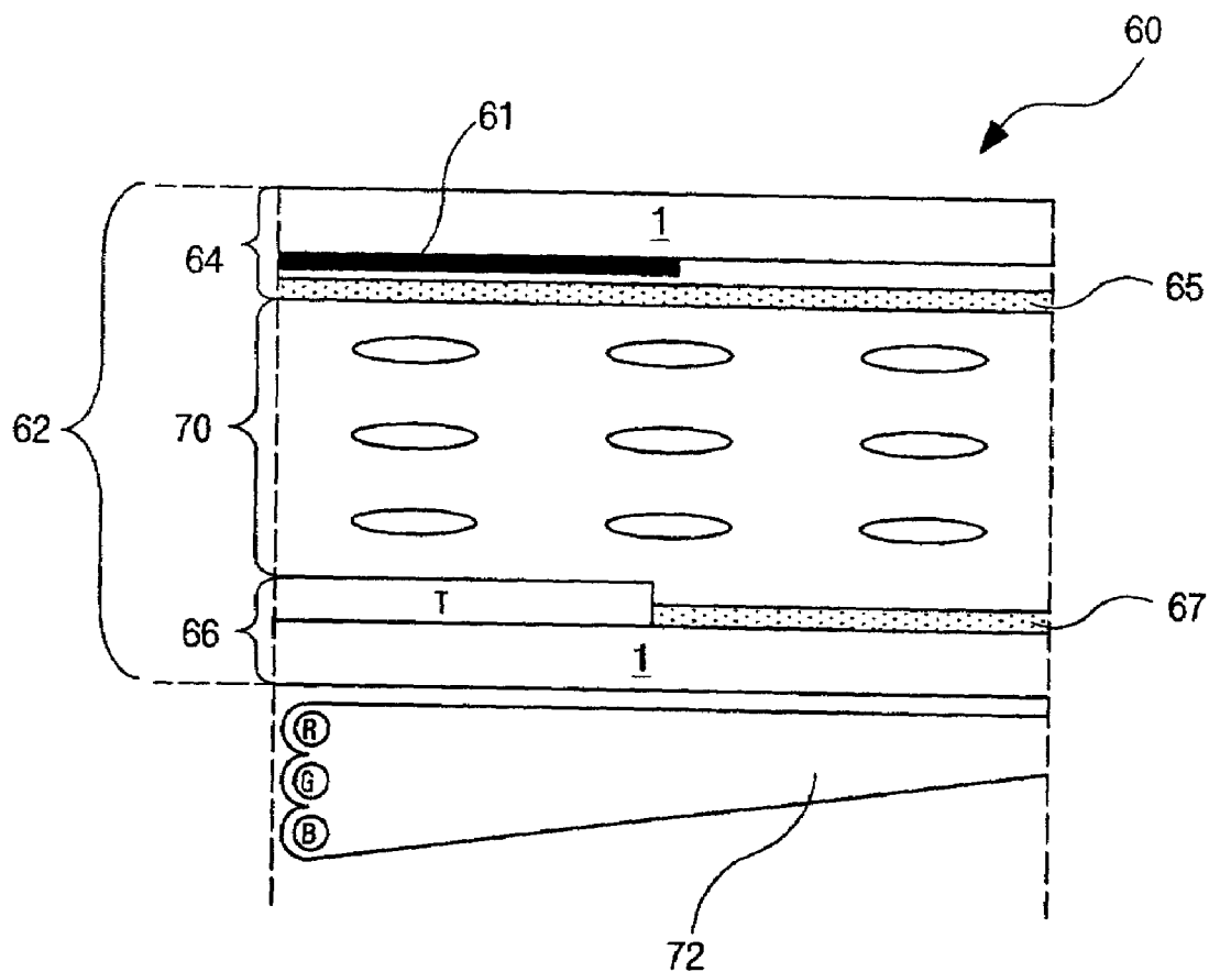
FIG. 2 (RELATED ART)
