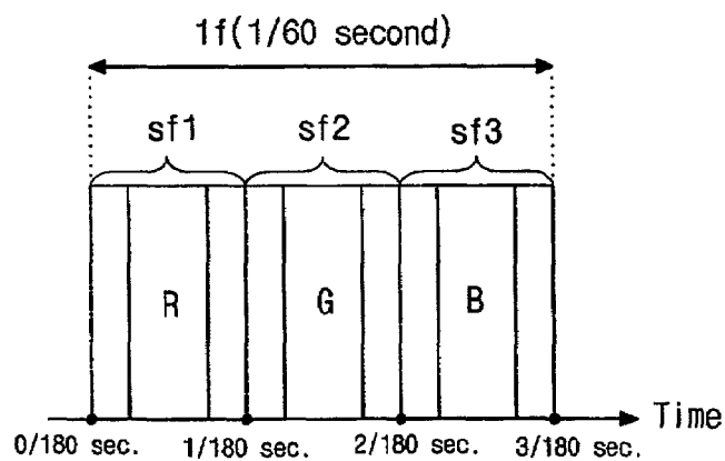
FIG. 5 (RELATED ART)
