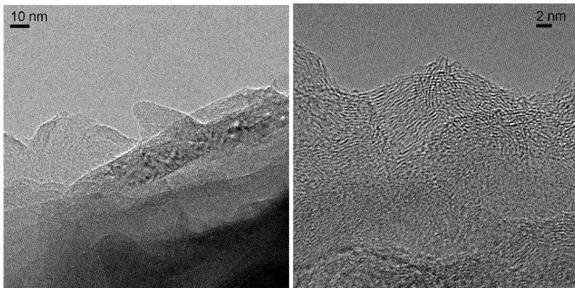
Figure 1: Transmission Electron Microscopy image of CVD coated GRAPHITE B
