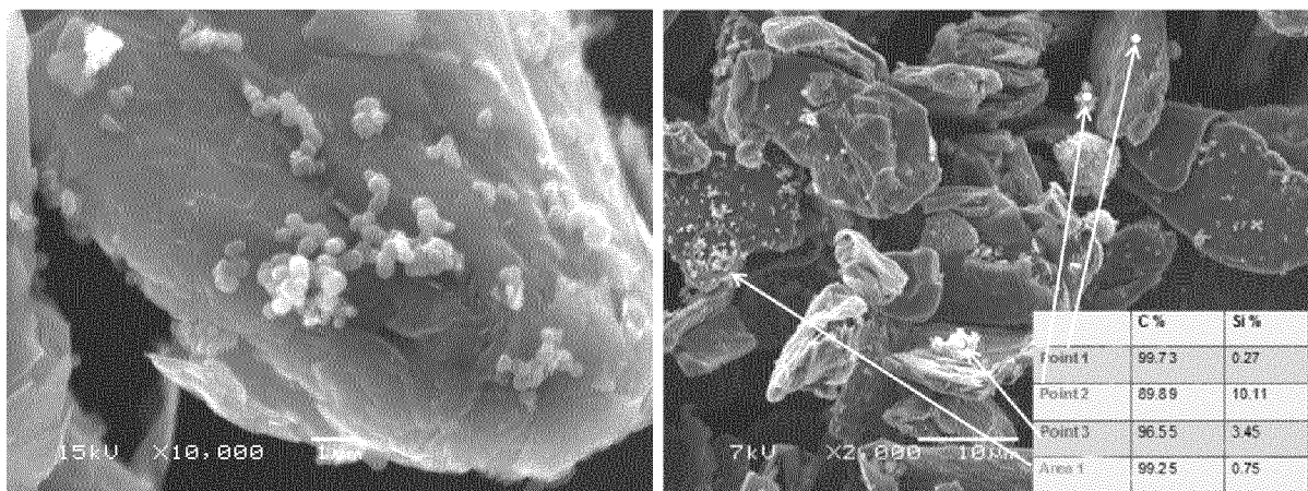
Figure 6: SEM image of a CVD-coated oxidized silicon/graphite composite material Si-C (left panel) and corresponding EDX analysis (right panel).
