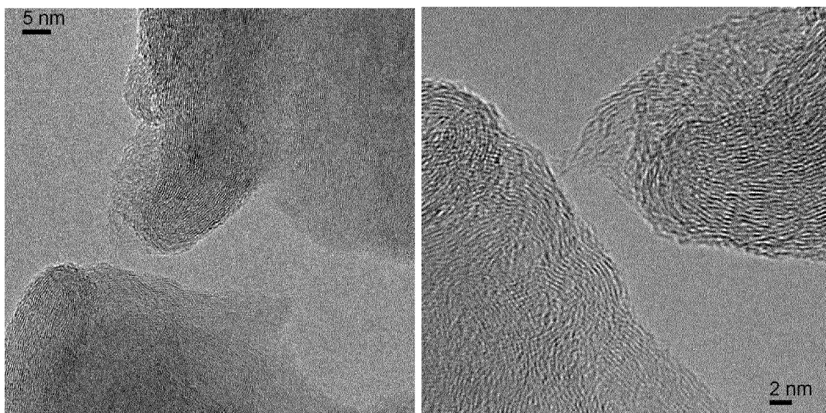
Figure 2: Transmission Electron Microscopy image of CVD coated and oxidized GRAPHITE B
