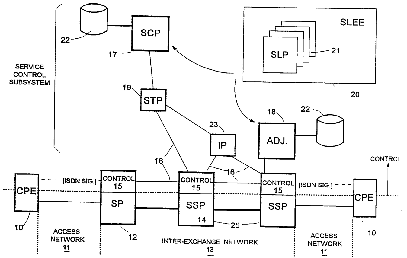
FIG. 2 (PRIOR ART)
