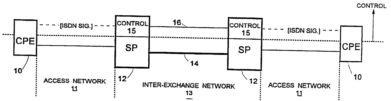
FIG. 1 (PRIOR ART)
