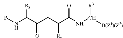
keto methylene isostere
