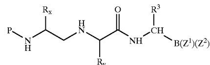
reduced peptide bond
