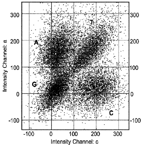
Phasing Corrected Intensities of Lane 1, Tile 2, Cycle 122
