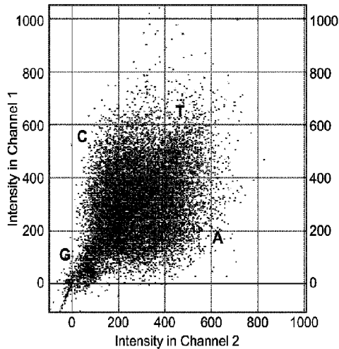
Raw Intensities of Lane 1, Tile 2, Cycle 122
