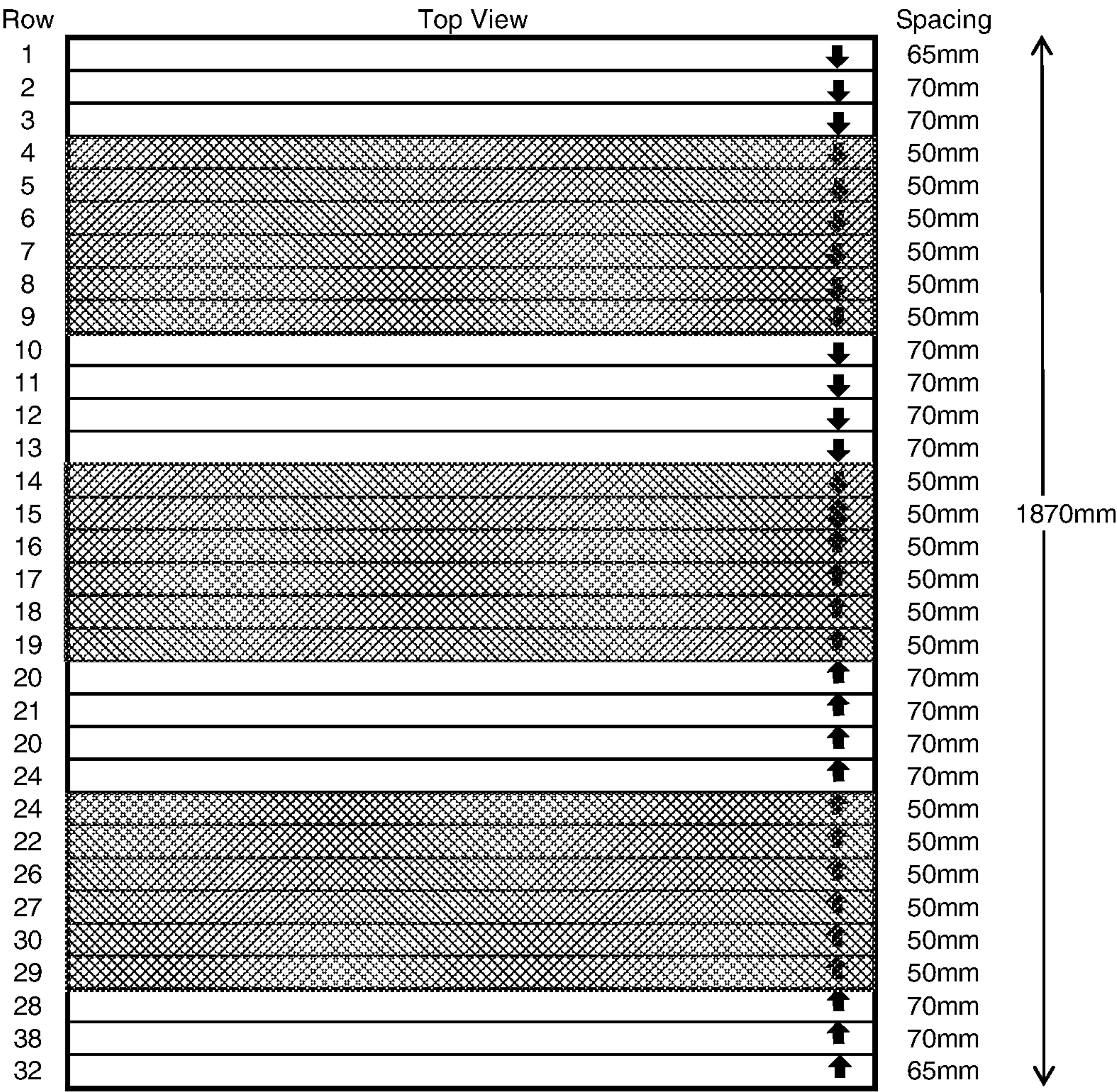
Ventilated Hole Spacings for Single & Double Size Mattress Cores.
