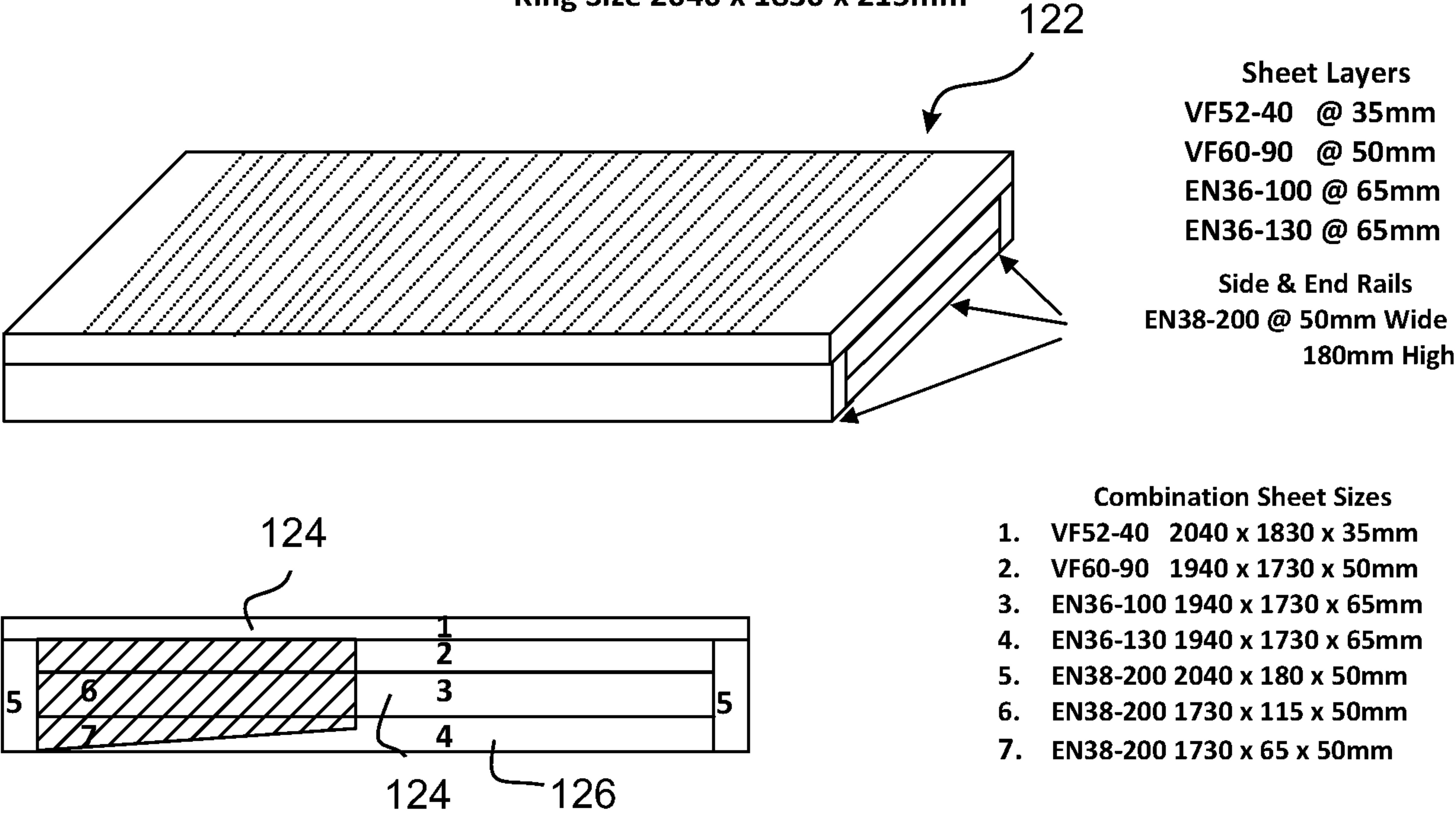
Fig. 9 7 Zone Ventilated Mattress Core with Side & End Support Rails EN36-100 Mid Layer Option King Size 2040 x 1830 x 215mm
