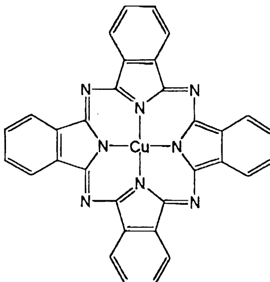
CuPc
