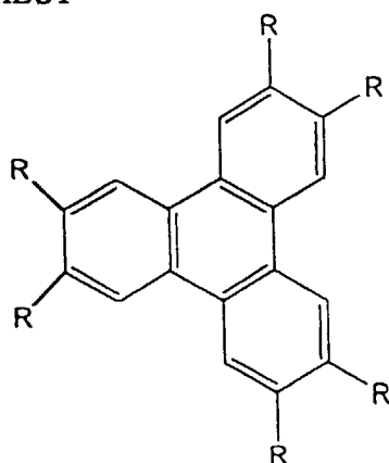
HBOT
