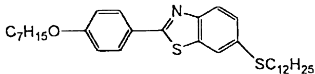
LC Compound 6
