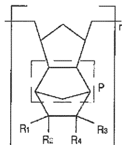
[Chemical Formula 4]
