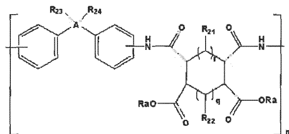
[Chemical Formula 6]
