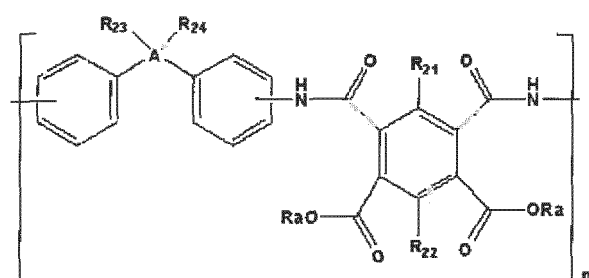
[Chemical Formula 5]
