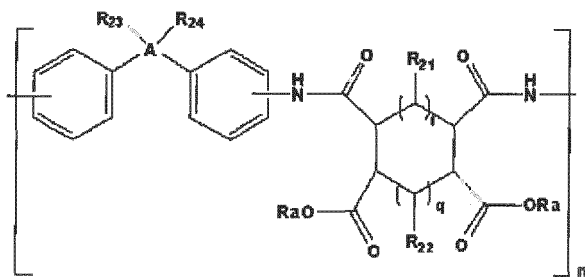
[Chemical Formula 6]
