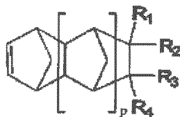
[Chemical Formula 2]
