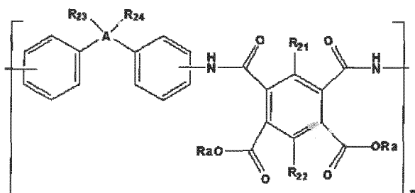
[Chemical Formula 6]
