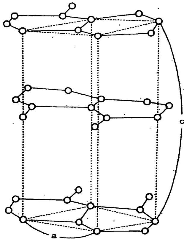
Fig.4, 7 Crystal Structure of Graphite
