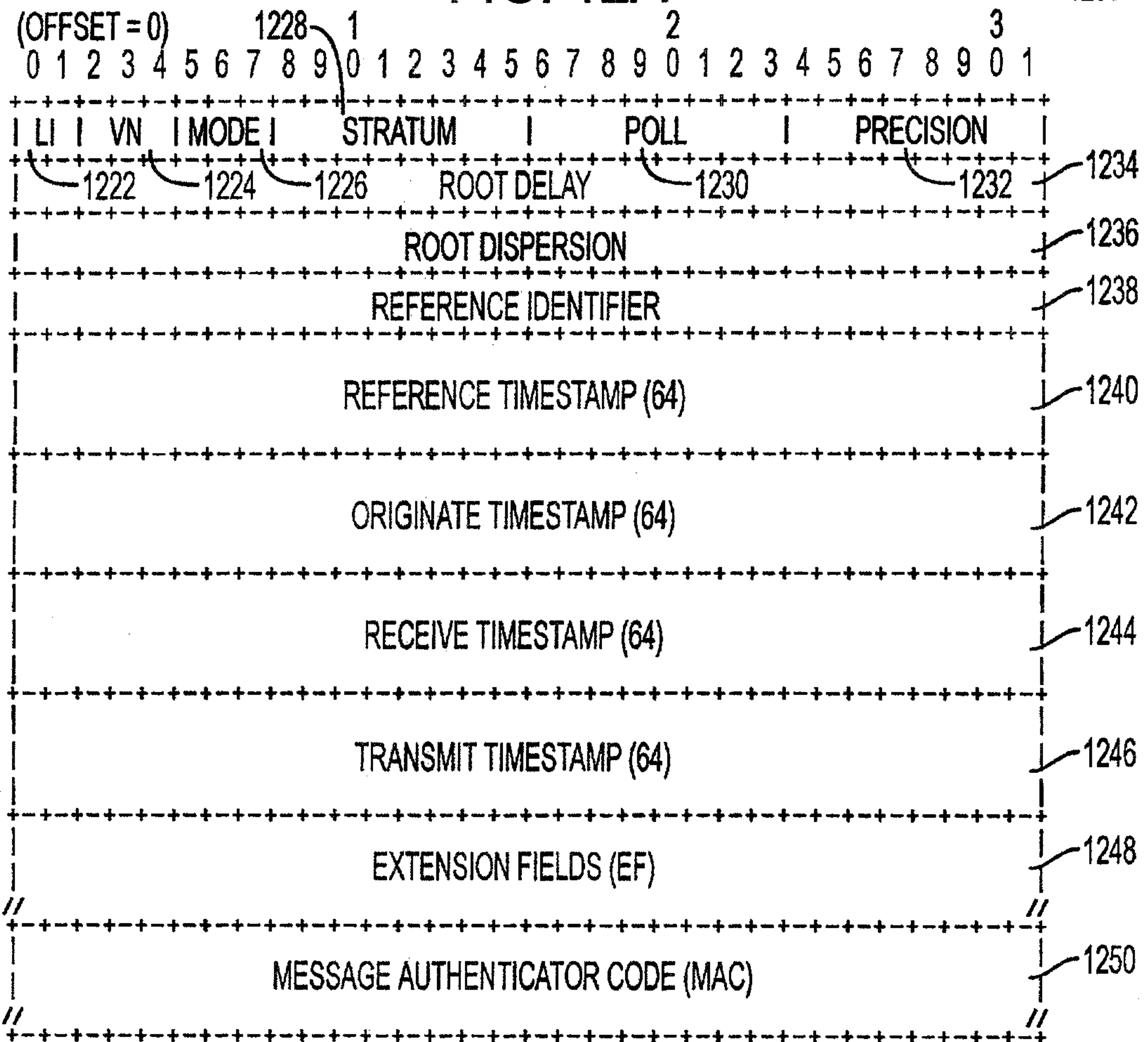
FIG. 12B (Prior Art)
