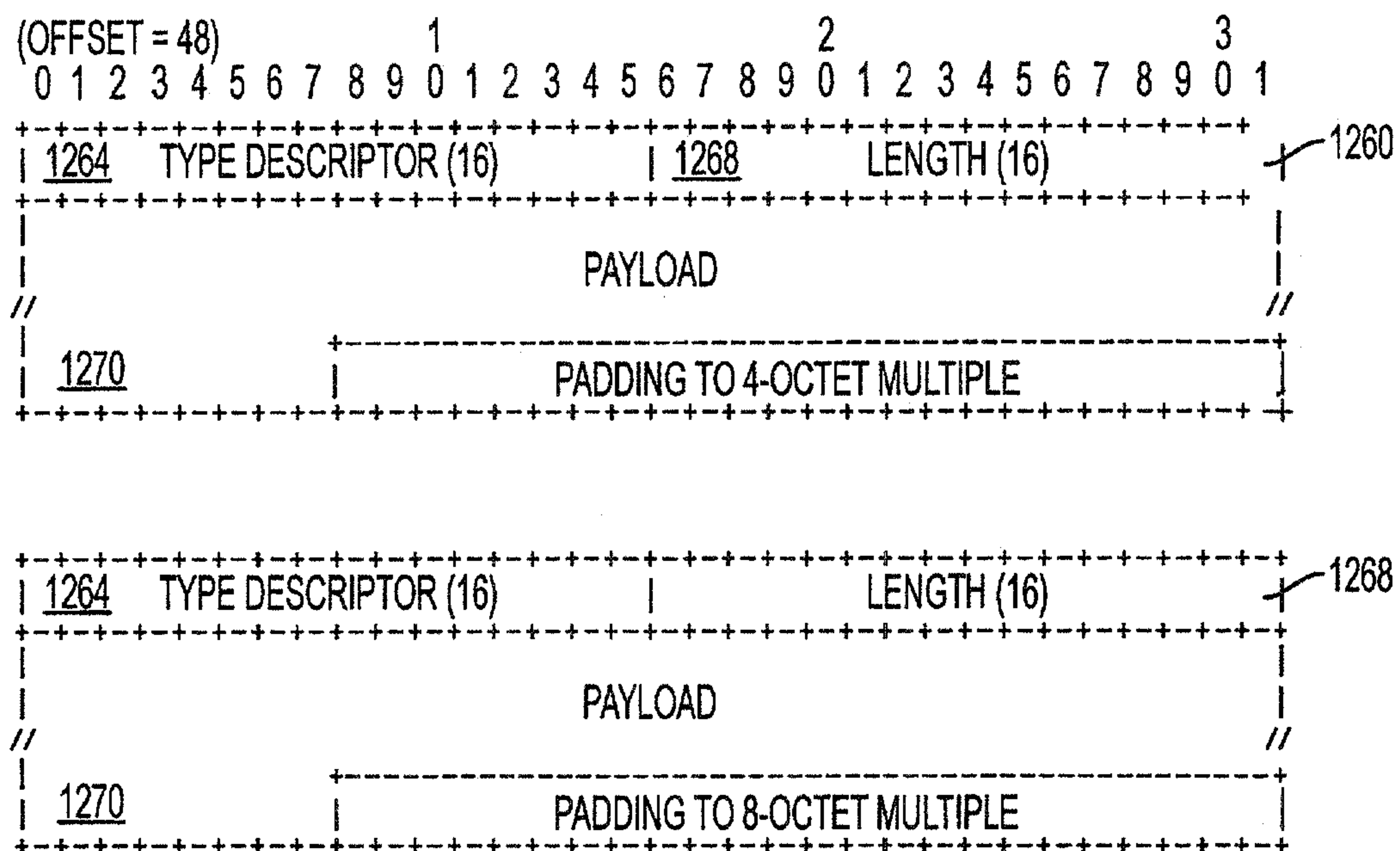
FIG. 12D (Prior Art)
