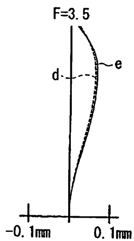
Spherical Aberration Fig. 3A
