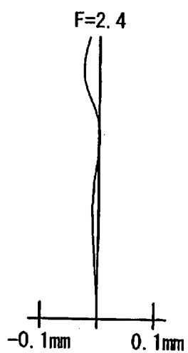
Spherical Aberration Fig. 4A
