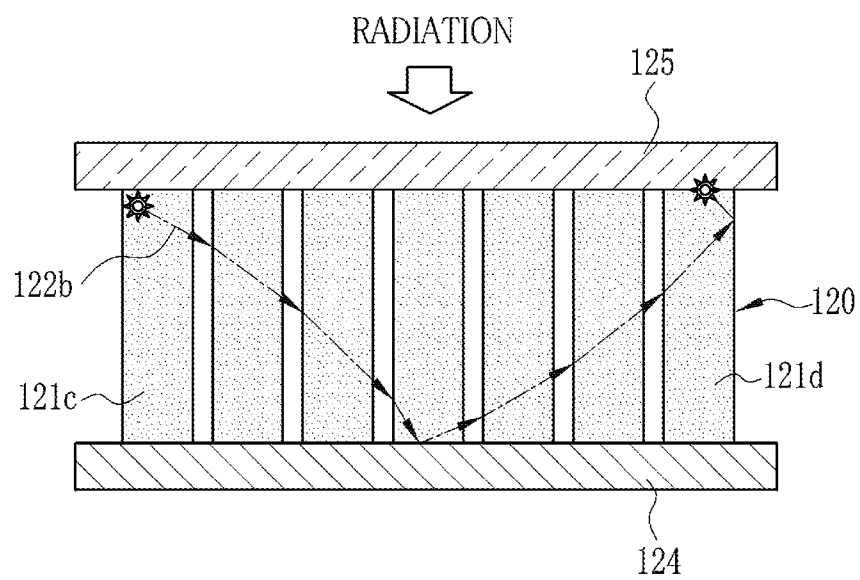
FIG. 19 (PRIOR ART)
