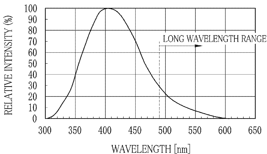
CsI (Na) EMISSION SPECTRUM
