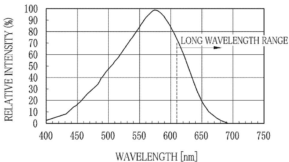
CsI (Ti) EMISSION SPECTRUM
