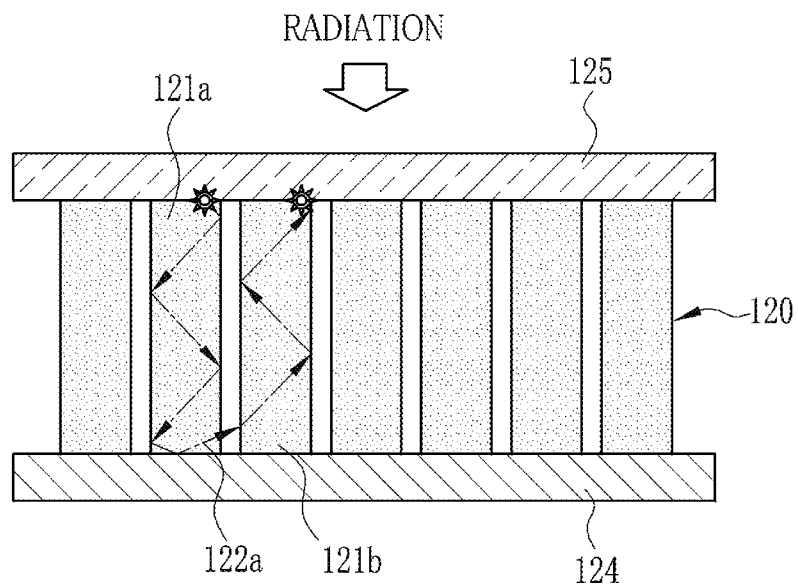
FIG. 18 (PRIOR ART)
