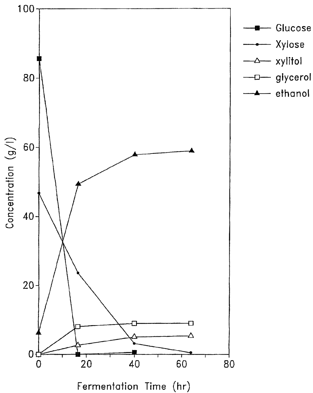
Fermentation of Glucose and Xylose by LNH32
