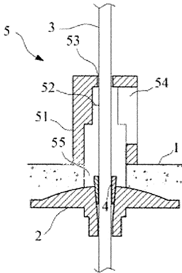
FIG. 1A (RELATED ART)
