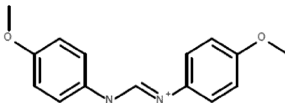
Anilinomethylene(phenyl)ammonium
