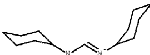
Cyclohexyl-[(cyclohexylamino)methylene]ammonium
