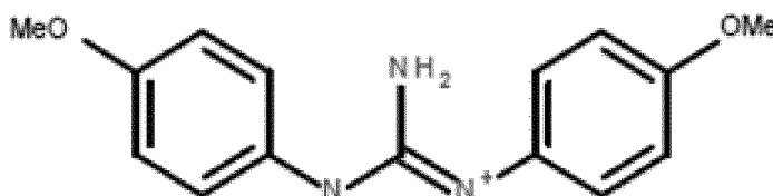
[Amino-(4-methoxyanilino)methylene]-(4-methoxyphenyl)ammonium
