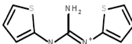
[Amino-(2-thienylamino)methylene]-(2-thienyl)ammonium
