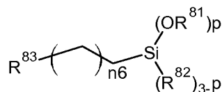
Structure (XIV)
