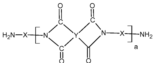
Structure (VIIIa)
