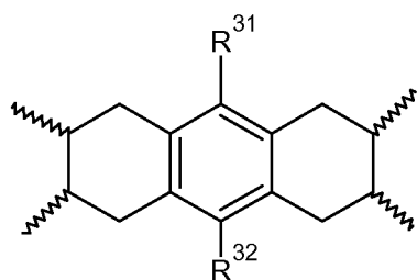
Structure (VI-a)
