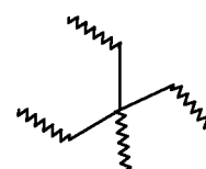
Structure (VI-j)
