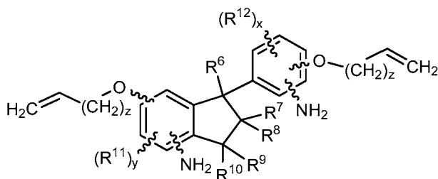
Structure (I)
