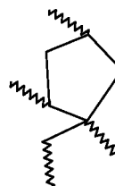
Structure (VI-i)
