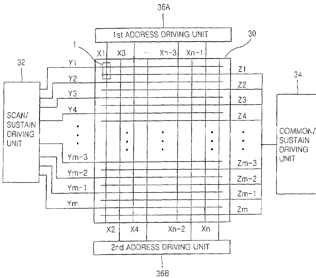
FIG. 2 CONVENTIONAL ART
