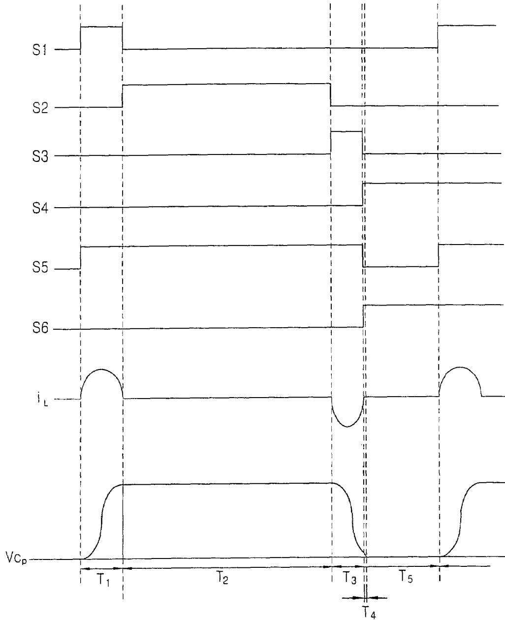
FIG. 6 CONVENTIONAL ART
