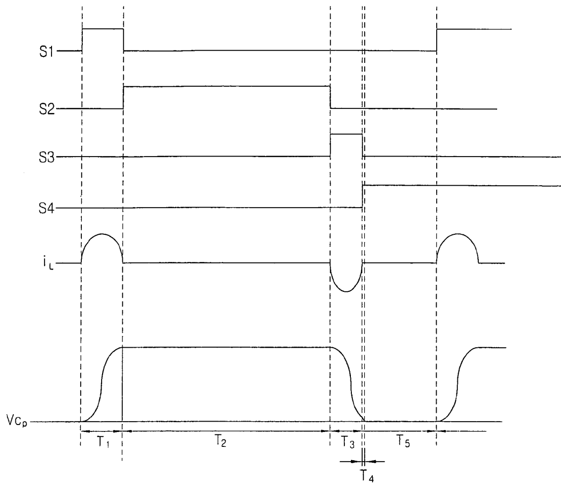
FIG. 4 CONVENTIONAL ART
