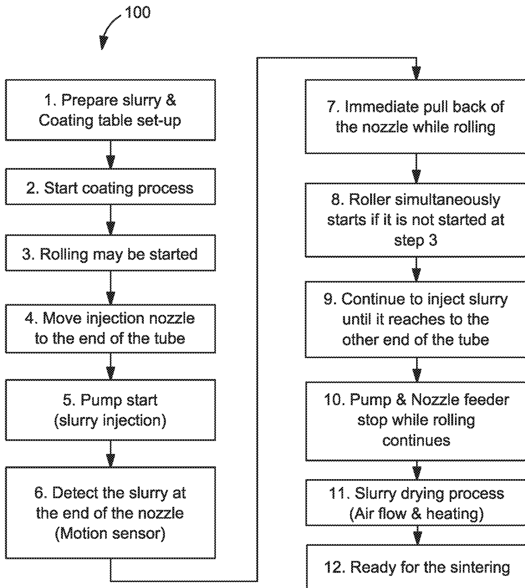
FIG. 1 Coating Process Map
