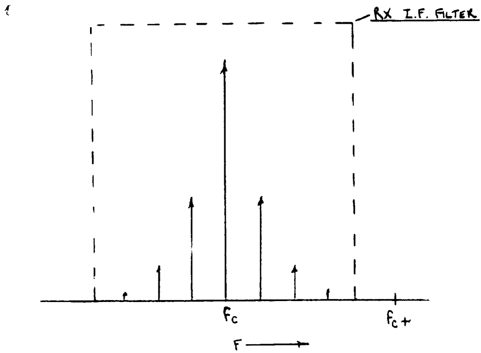
FIG 2 a SIDEBAND STRUCTURE OF WANTED SIGNAL
