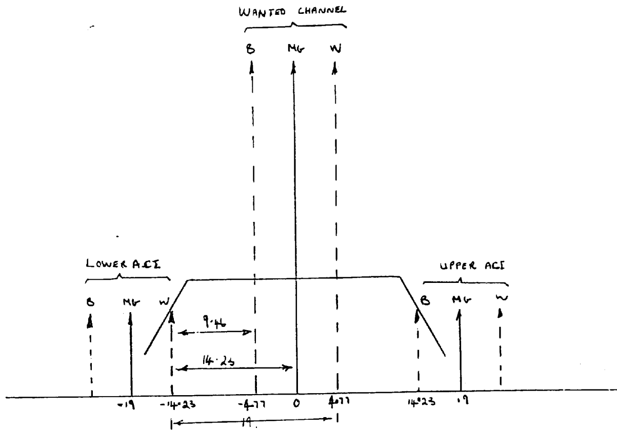
FIG 1 STATIC TONE INTERFERENCE
