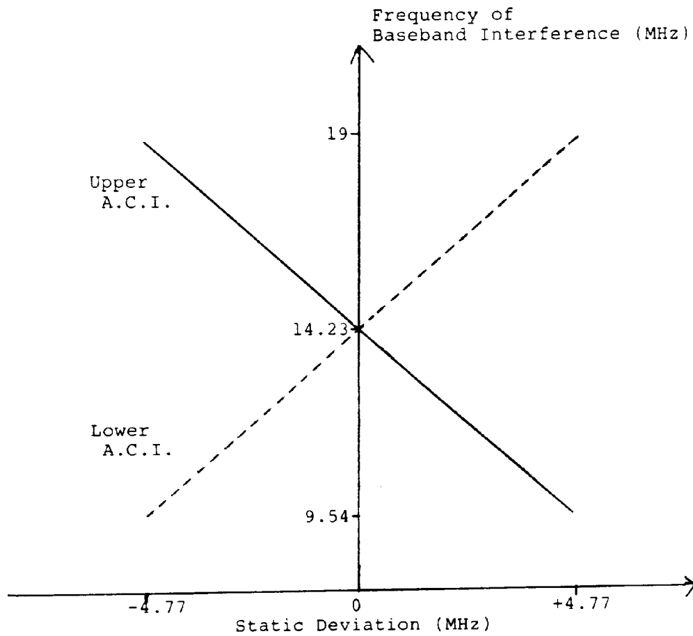
FIG.5 Lowest Frequency Possible for Static Tone Interference Versus Static Deviation of Wanted Channel
