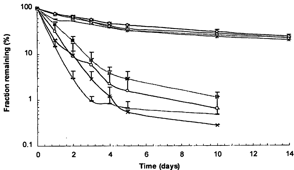
Stability of ICG in free aqueous solutions and in nanoparticles suspended in water (initial concentration = 0.001 mg/ml) (n = 3 for each data point)
