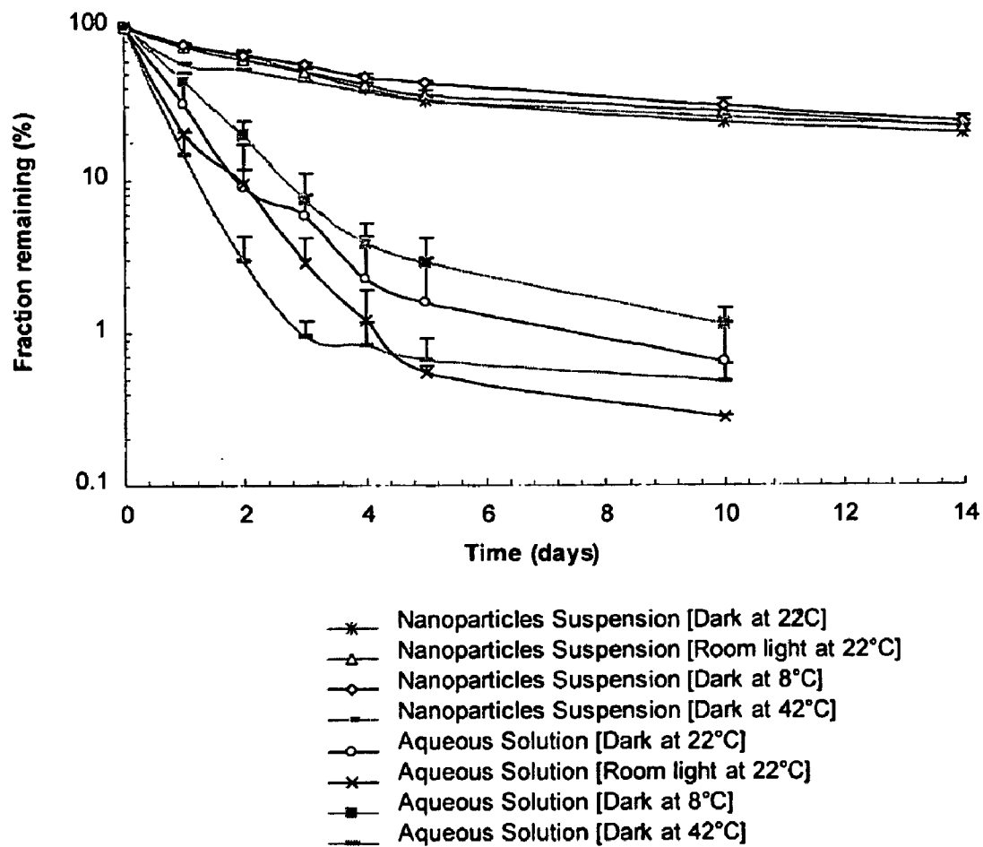
Stability of ICG in free aqueous solutions and in nanoparticles suspended in water (initial concentration = 0.001 mg/ml) (n = 3 for each data point)
