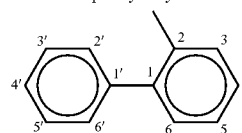
biphenyl-3-yl-
