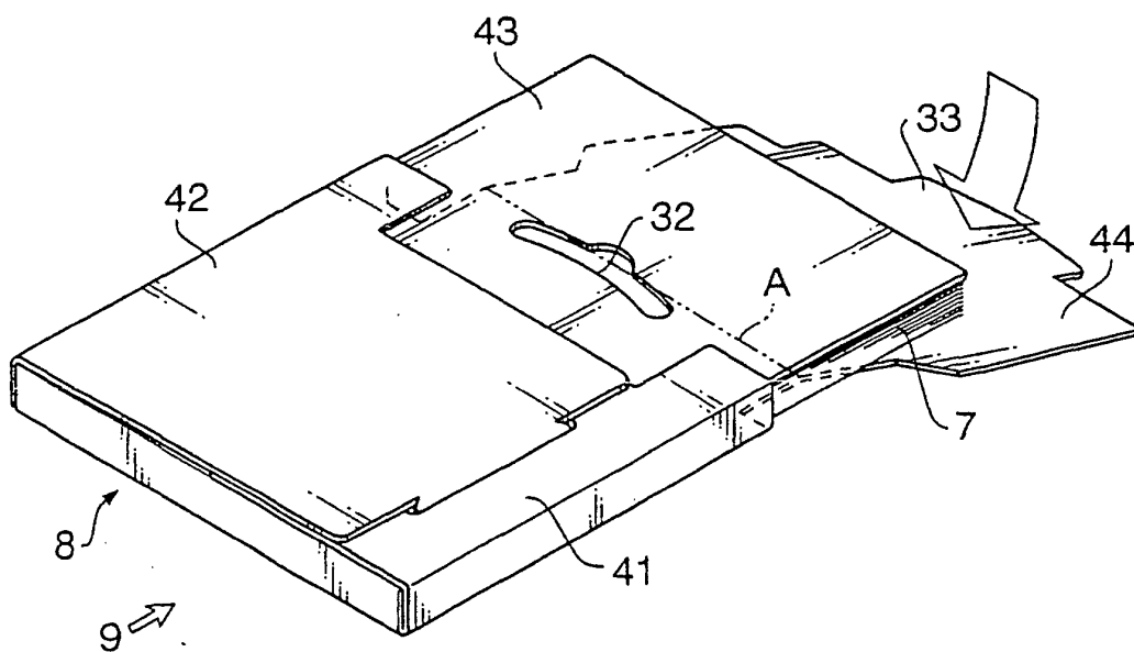
FIG 14 PROCESS FOR SETTING PACKAGE IN PRINTER: 3
