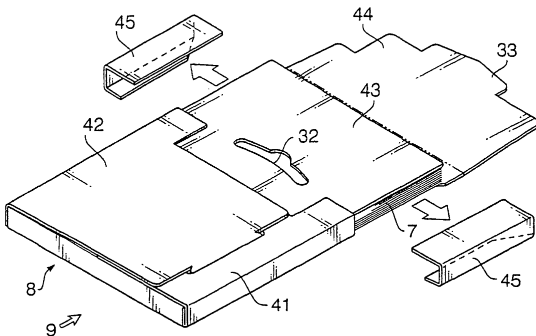
FIG 13 PROCESS FOR SETTING PACKAGE IN PRINTER: 2
