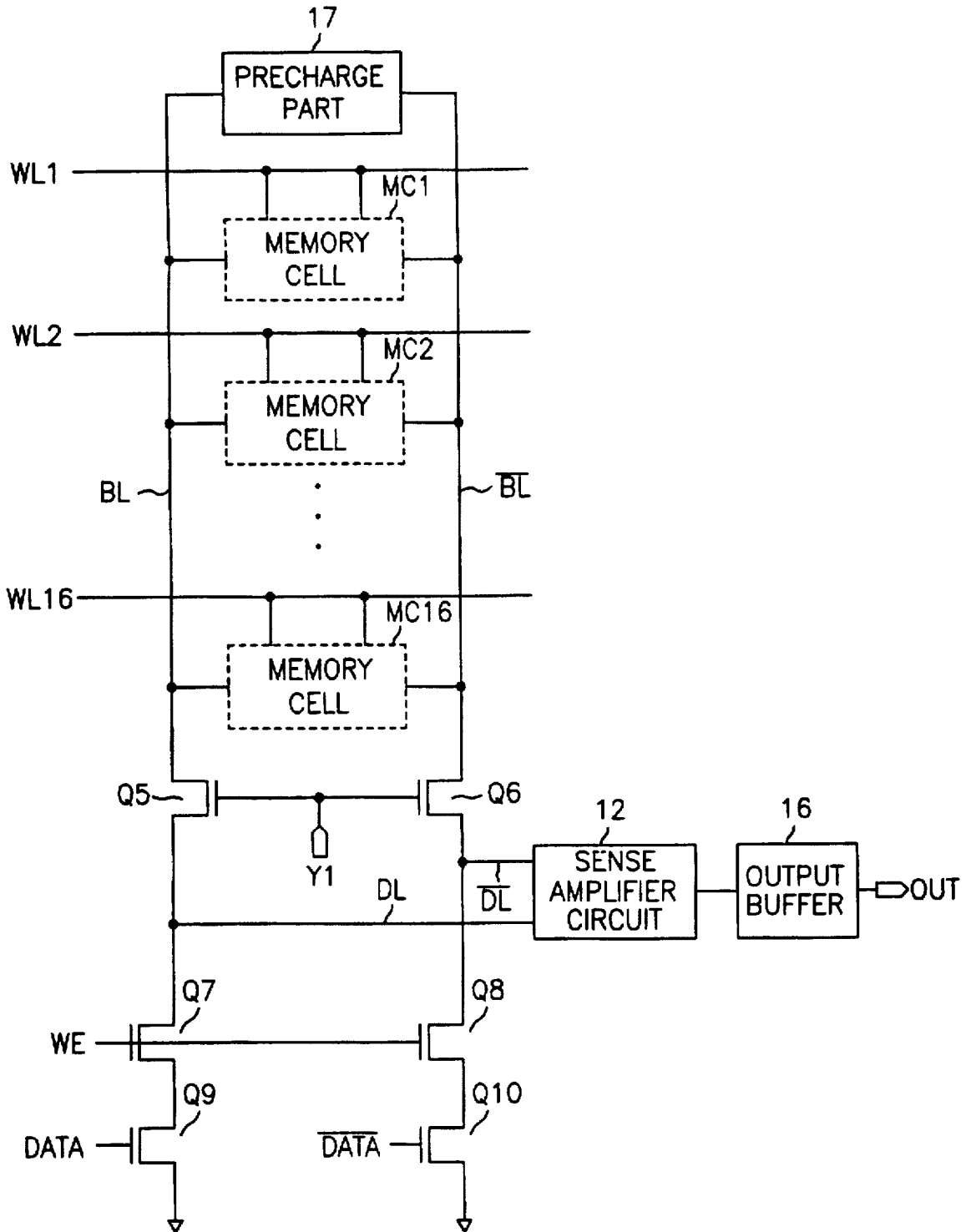
FIG. 3 (PRIOR ART)
