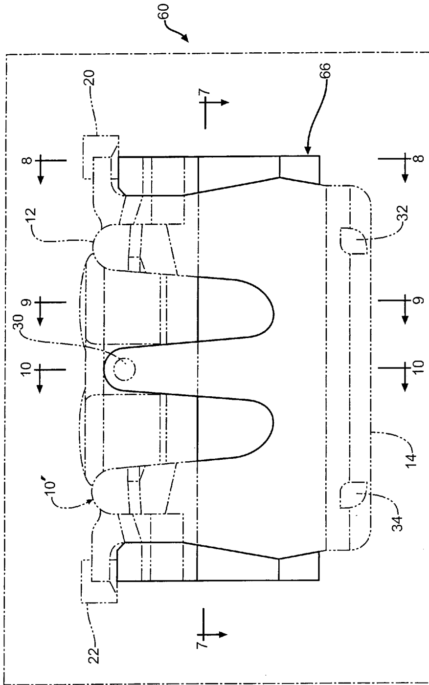
FIG. 6 (PRIOR ART)
