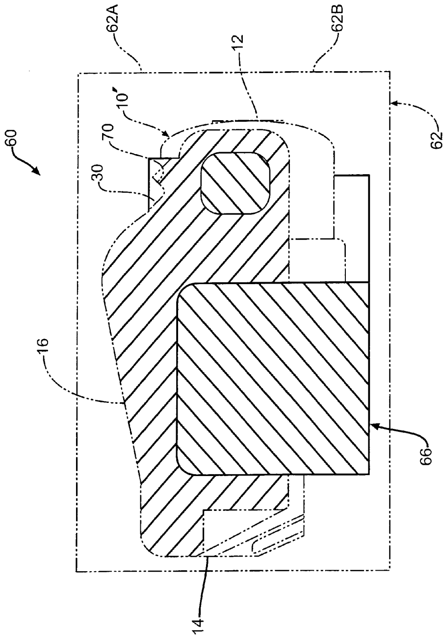
FIG. 10 (PRIOR ART)
