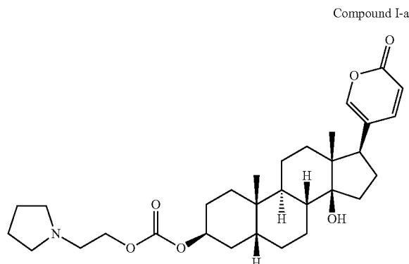
Compound I-a
