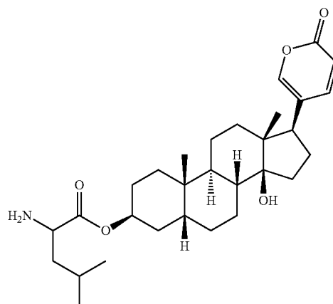
Compound II-c
