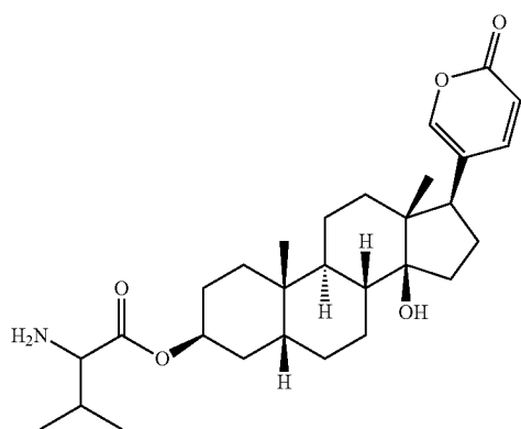
Compound II-b
