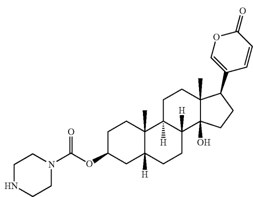
Compound I-e
