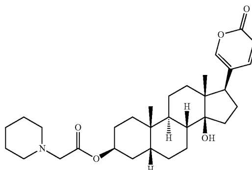
Compound II-e
