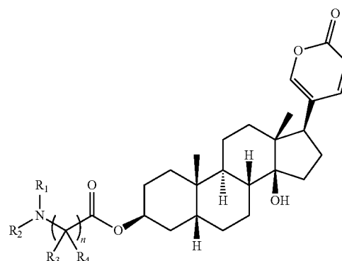
Formula II
