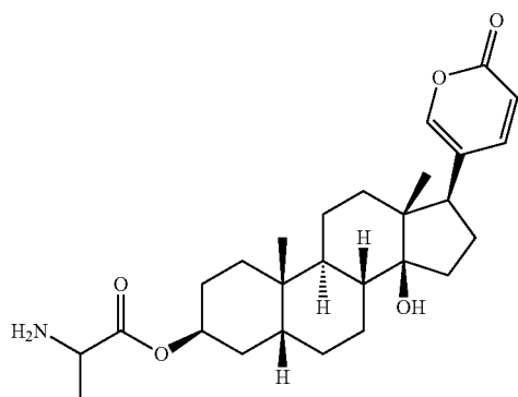
Compound II-a
