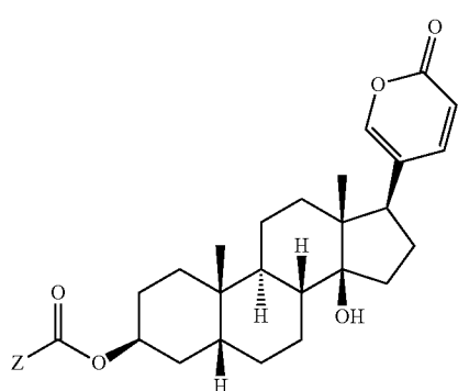
Formula I
