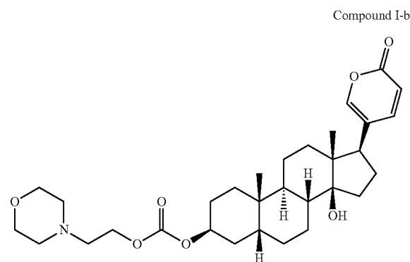
Compound I-b
