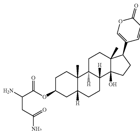
Compound II-d
