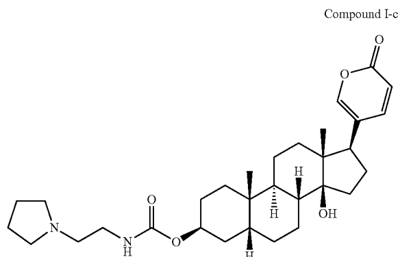
Compound I-c
