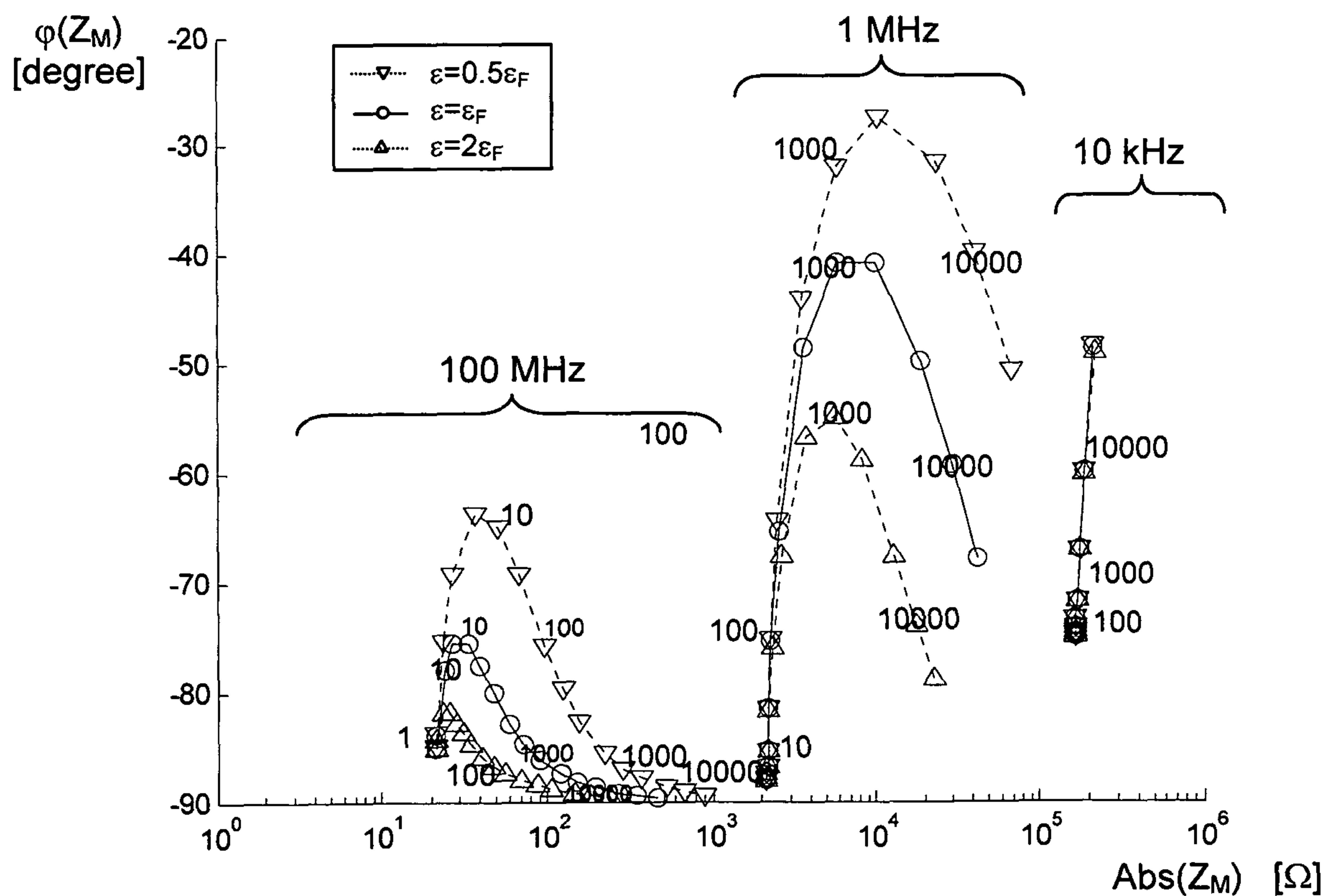
FIG. 2 - PRIOR ART
