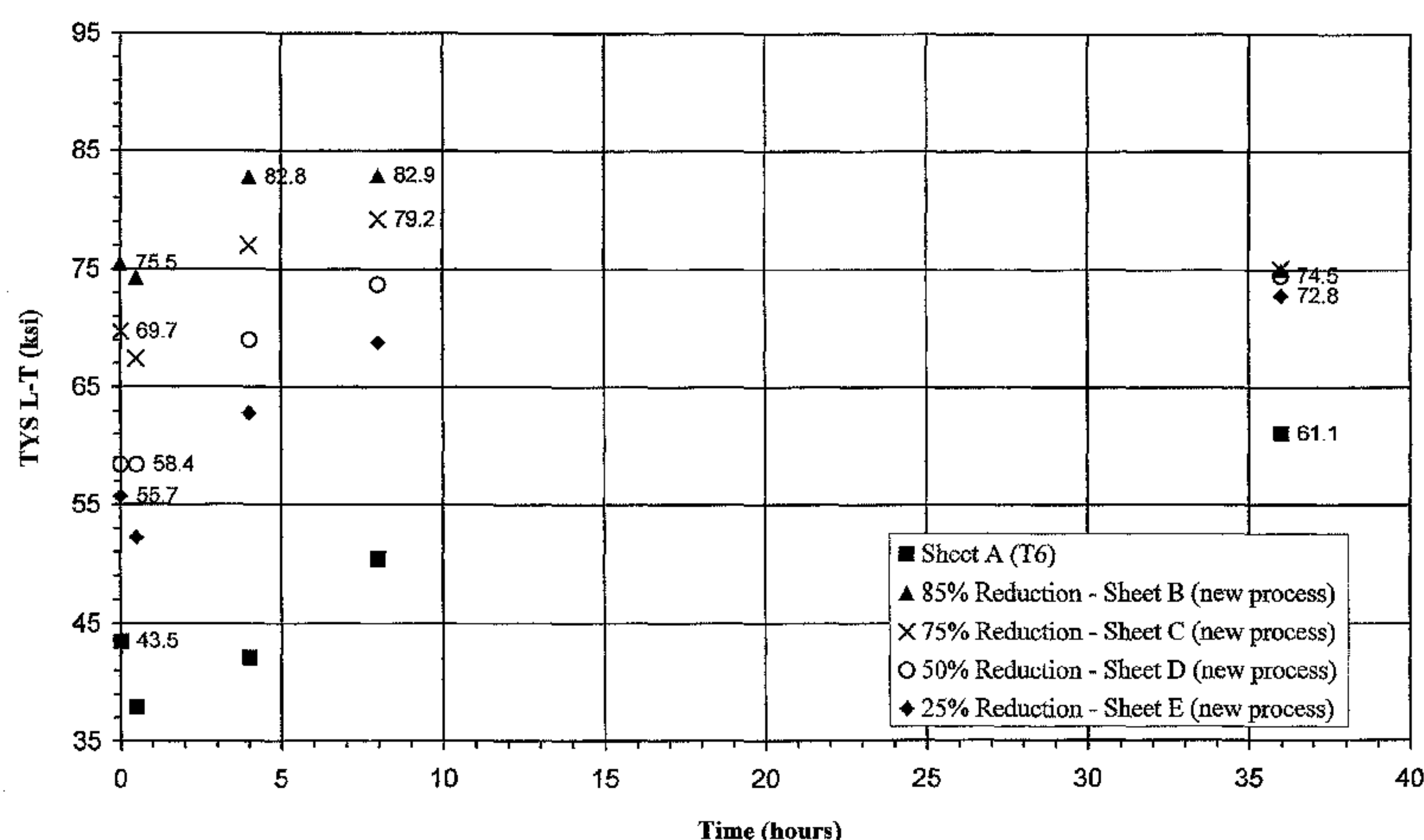
FIG. 15 - 2xxx+Ag - TYS v. Time at 330F
