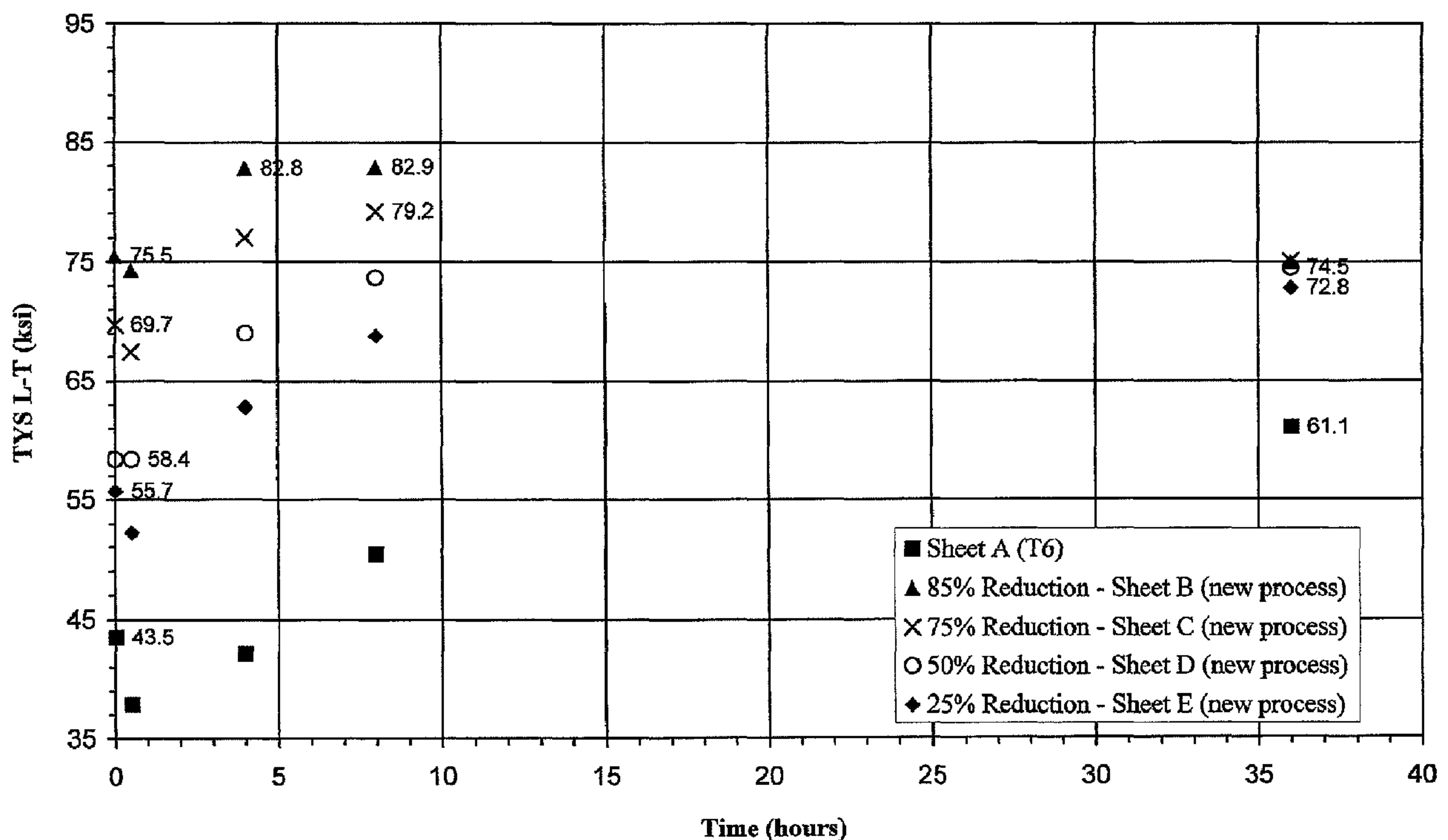
FIG. 15 - 2xxx+Ag - TYS v. Time at 330F
